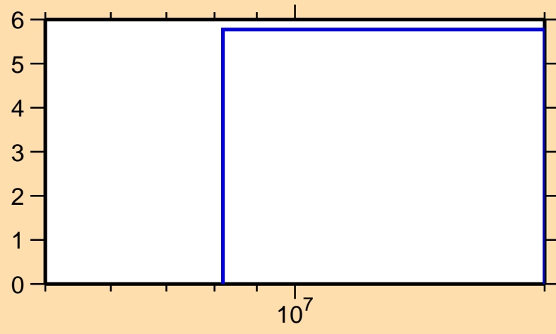
\Delta\sigma/\sigma vs. E for ^{134}\text{Te}(n,el.)
