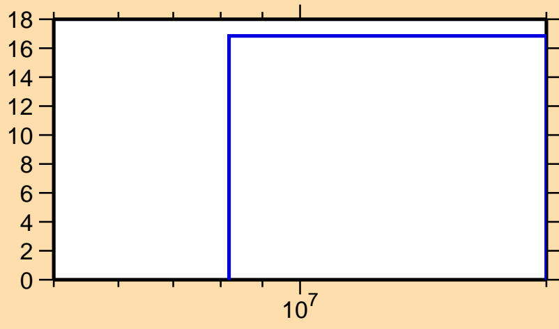
\Delta\sigma/\sigma vs. E for ^{134}\text{Te}(n,n\text{cont.})
