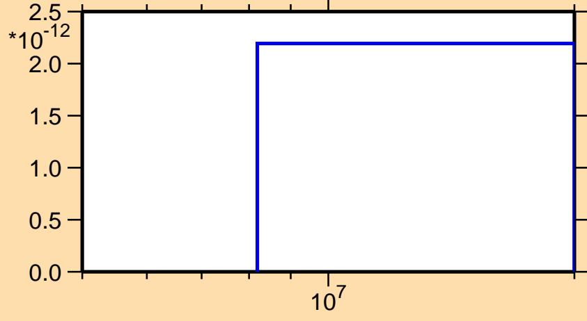
\sigma vs. E for ^{134}\text{Te}(n,\text{nd})
