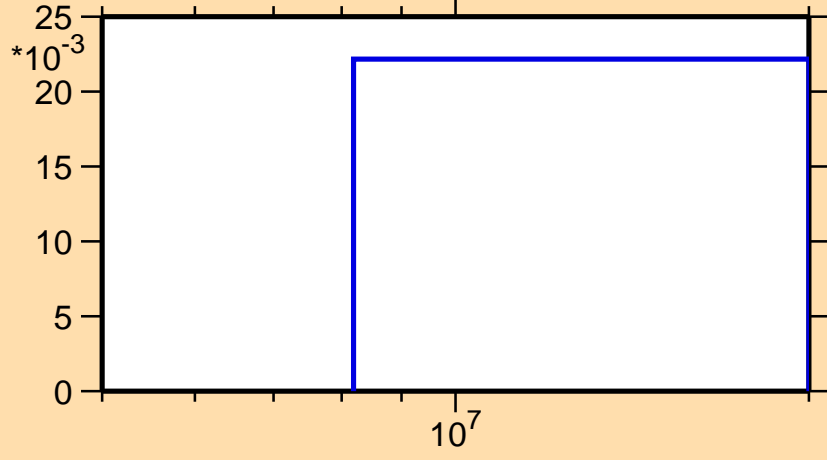
\sigma vs. E for ^{134}\text{Te}(n,3n)
