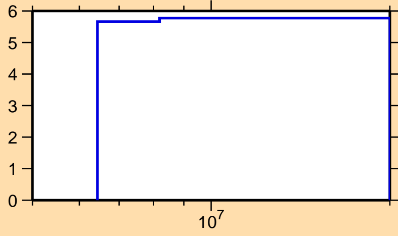
\Delta\sigma/\sigma vs. E for ^{134}\text{Te}(n,\text{el.})
