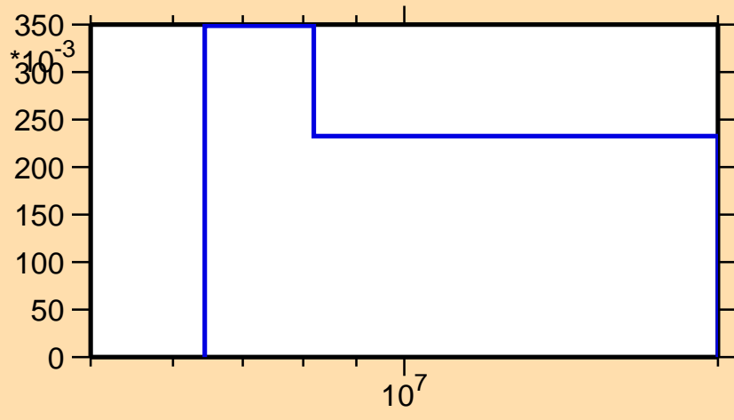
\sigma vs. E for ^{134}\text{Te}(n,n\text{cont.})
