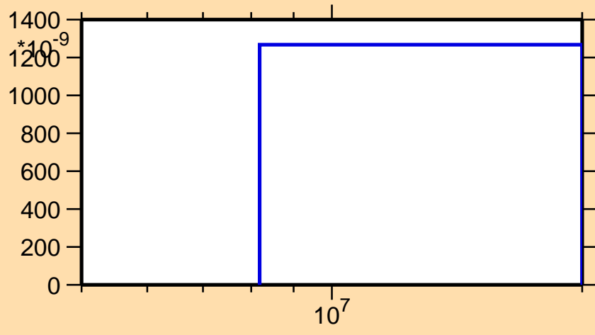
\sigma vs. E for ^{134}\text{Te}(n,t)
