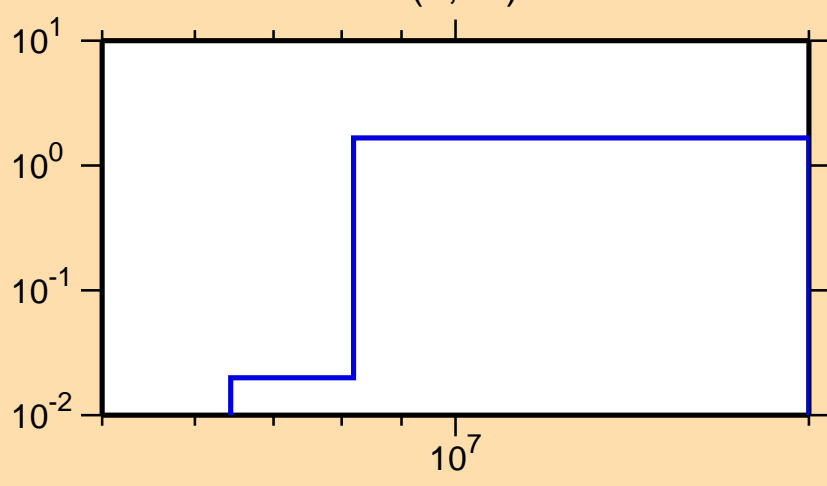
\sigma vs. E for ^{134}\text{Te}(n,2n)
