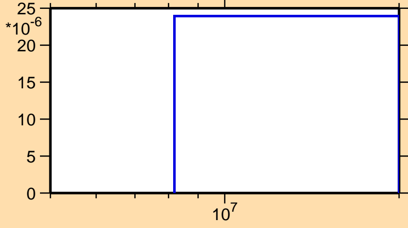
\sigma vs. E for ^{134}\text{Te}(n,d)
