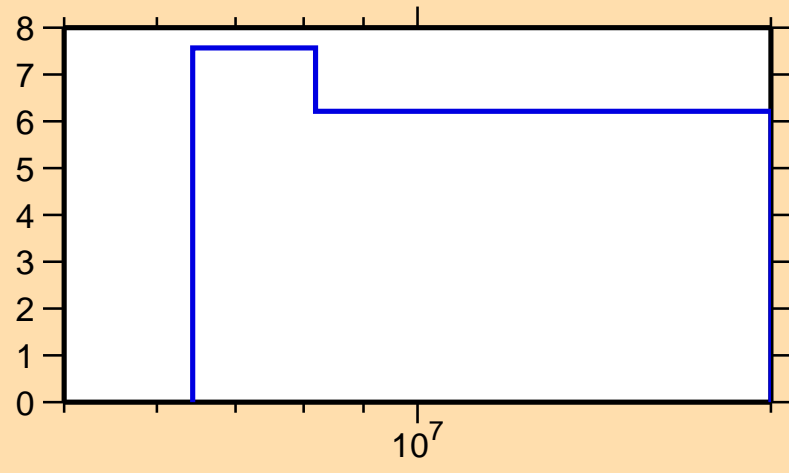
\Delta\sigma/\sigma vs. E for ^{134}\text{Te}(n,\text{inel.})
