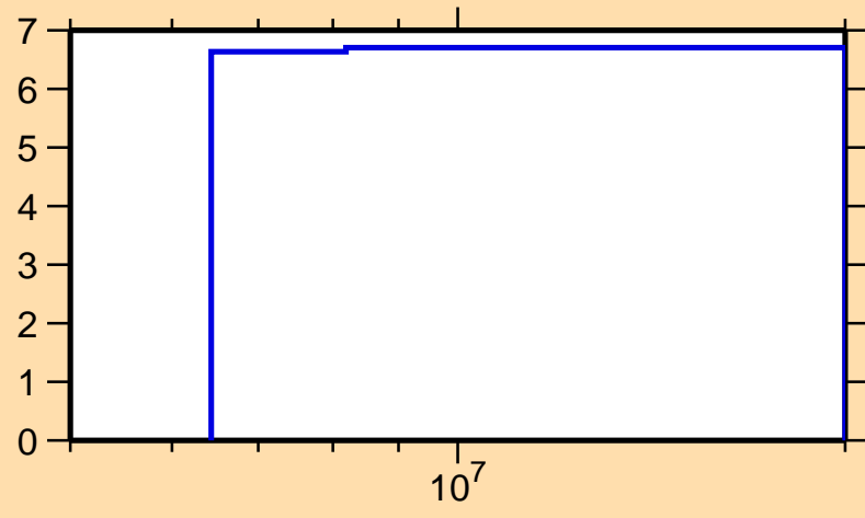
\Delta\sigma/\sigma vs. E for ^{134}\text{Te}(n,\text{nonel.})
