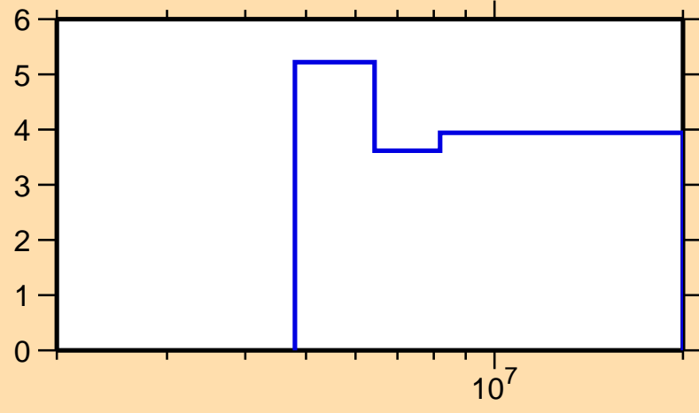
\Delta\sigma/\sigma vs. E for ^{134}\text{Te}(n,\text{tot.})
