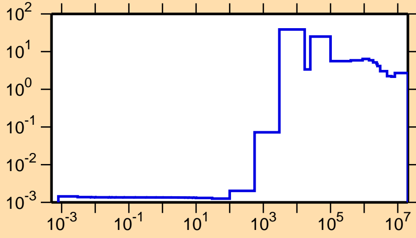
\sigma vs. E for ^{134}\text{Te}(n,\text{el.})
