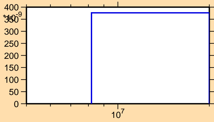
\sigma vs. E for ^{134}\text{Te}(n,n\alpha)
