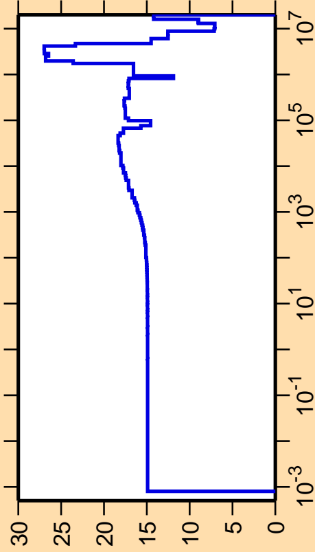
\Delta\sigma/\sigma vs. E for ^{136}\text{Te}(n,\text{el.})
