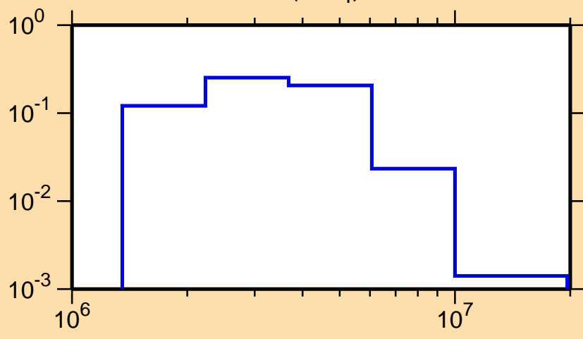
\sigma vs. E for ^{136}\text{Te}(n,n_4)
