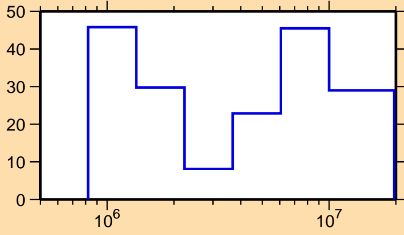
\Delta\sigma/\sigma vs. E for ^{136}\text{Te}(n,\text{inel.})
