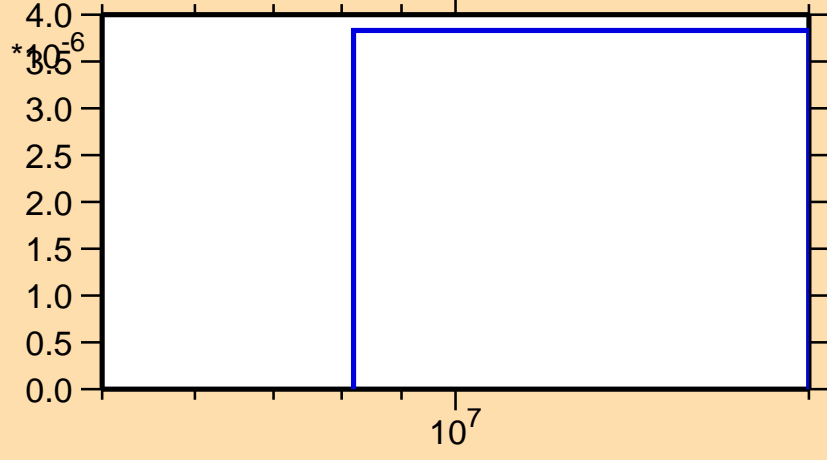
\sigma vs. E for ^{136}\text{Te}(n,d)
