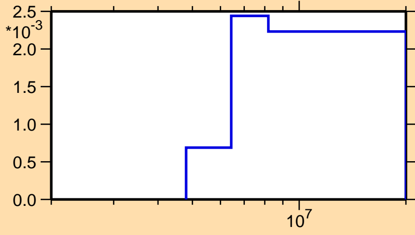
\sigma vs. E for ^{136}\text{Te}(n,n\text{cont.})
