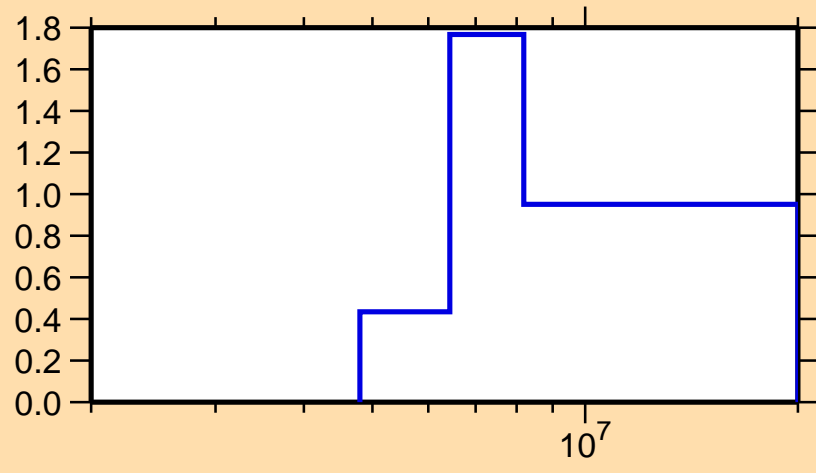
\sigma vs. E for ^{136}\text{Te}(n,2n)
