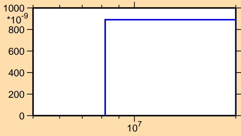
\sigma vs. E for ^{136}\text{Te}(n,np)
