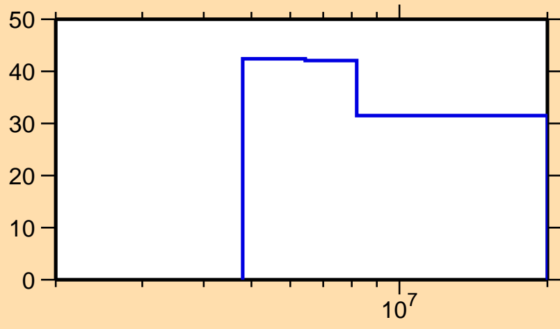
\Delta\sigma/\sigma vs. E for ^{136}\text{Te}(n,n_1)
