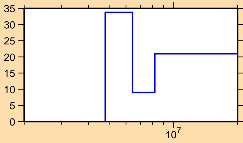
\Delta\sigma/\sigma vs. E for ^{136}\text{Te}(n,2n)
