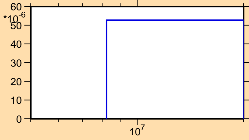
\sigma vs. E for ^{136}\text{Te}(n,t)
