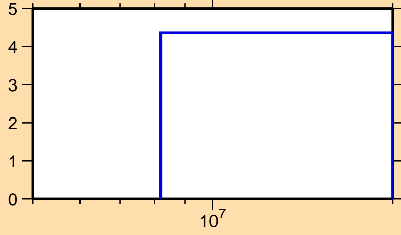
\Delta\sigma/\sigma vs. E for ^{136}\text{Te}(n,\text{tot.})
