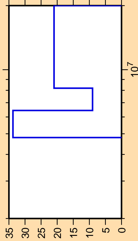
\Delta\sigma/\sigma vs. E for ^{136}\text{Te}(n,2n)
