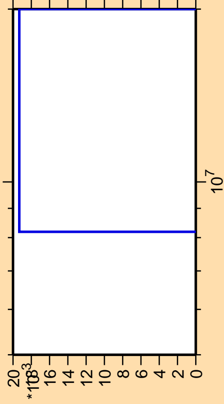
\Delta\sigma/\sigma vs. E for ^{136}\text{Te}(\text{mt } 11)
