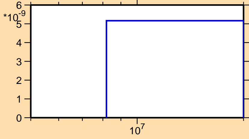
\sigma vs. E for ^{136}\text{Te}(n,nd)
