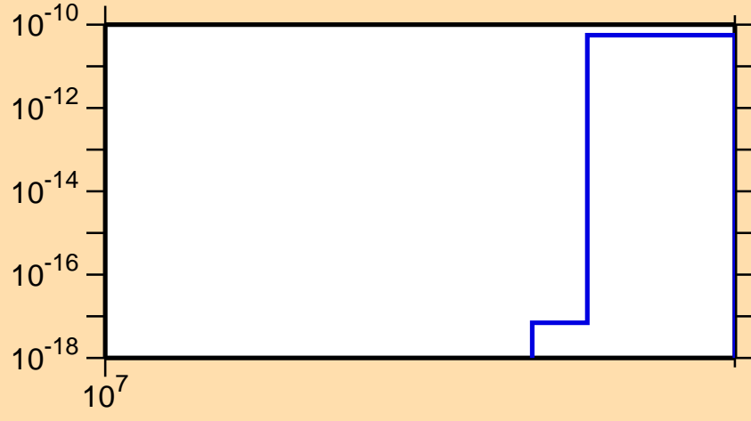
\sigma vs. E for ^{138}\text{Te}(n,2np)
