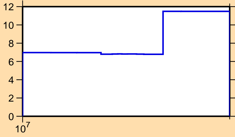
\Delta\sigma/\sigma vs. E for ^{138}\text{Te}(n,el.)
