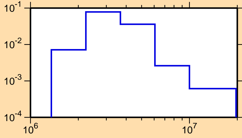
\sigma vs. E for ^{138}\text{Te}(n,n_3)
