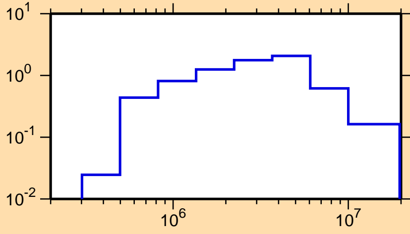
\sigma vs. E for ^{138}\text{Te}(n,\text{inel.})
