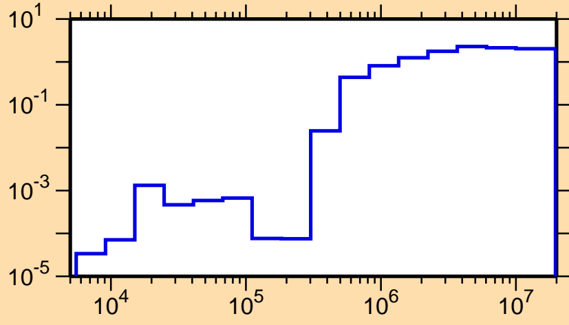
\sigma vs. E for ^{138}\text{Te}(n,\text{nonel.})
