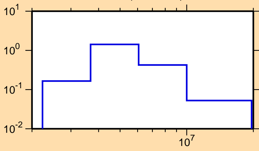
\sigma vs. E for ^{138}\text{Te}(n,n\text{cont.})
