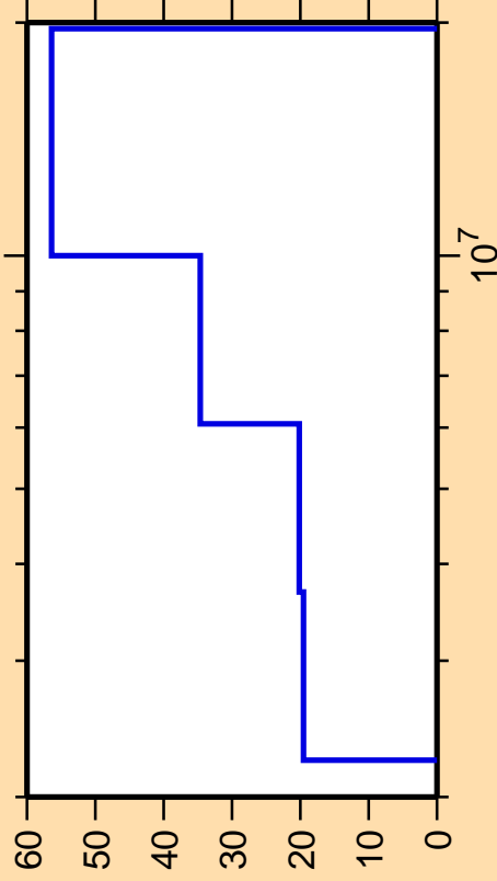
\Delta\sigma/\sigma vs. E for ^{138}\text{Te}(n,n\text{cont.})
