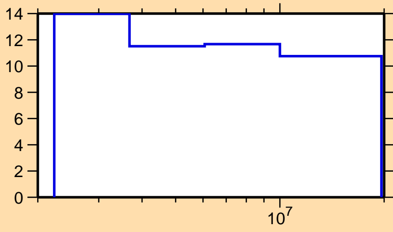
\Delta\sigma/\sigma vs. E for ^{138}\text{Te}(n,n\text{onel.})
