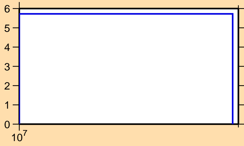
\Delta\sigma/\sigma vs. E for ^{138}\text{Te}(n,el.)
