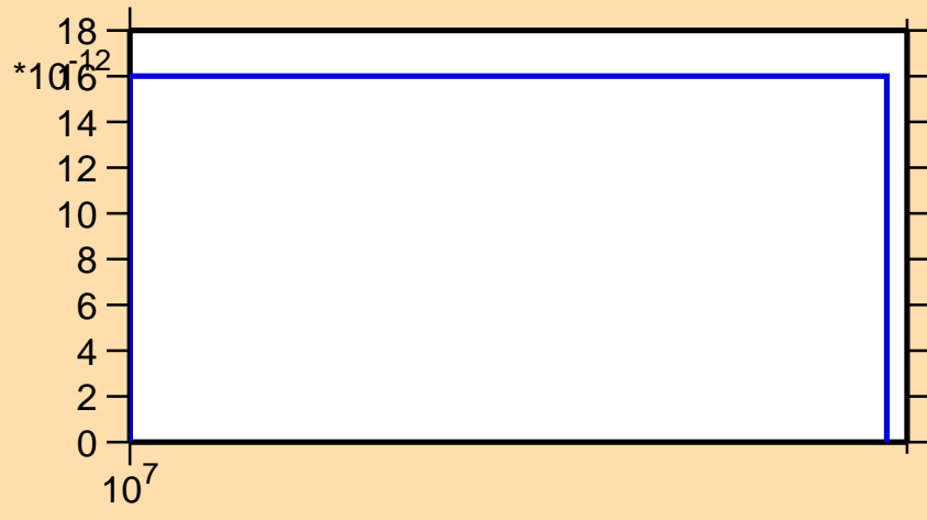
\sigma vs. E for ^{138}\text{Te}(n,3n\alpha)
