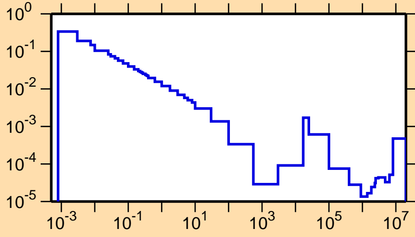
\sigma vs. E for ^{138}\text{Te}(n,\gamma)
