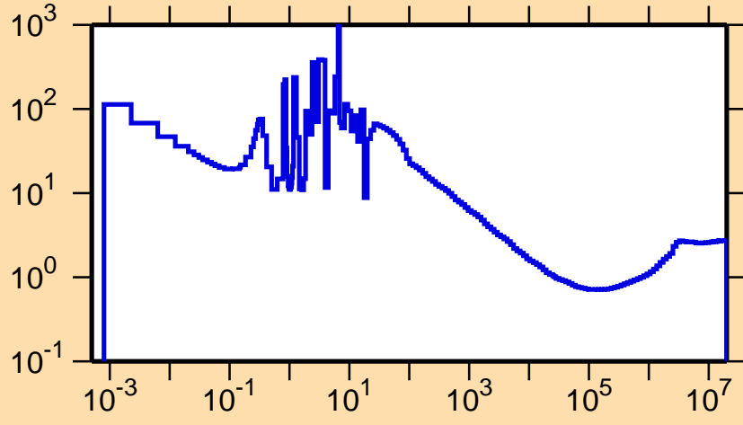
\sigma vs. E for ^{225}\text{Th}(n,\text{nonel.})
