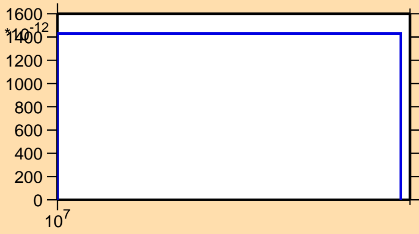
\sigma vs. E for ^{225}\text{Th} (mt 45)
