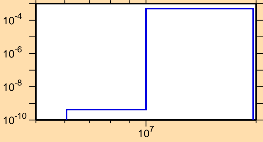
\sigma vs. E for ^{225}\text{Th}(n,np)
