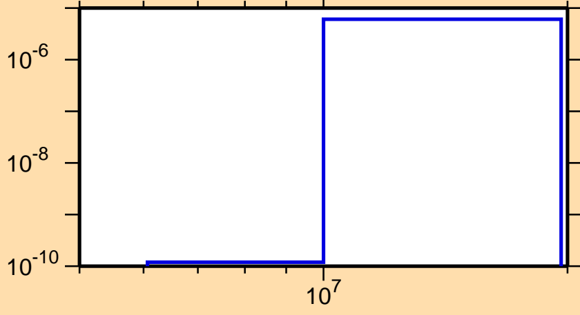
\sigma vs. E for ^{225}\text{Th}(n,p\alpha)
