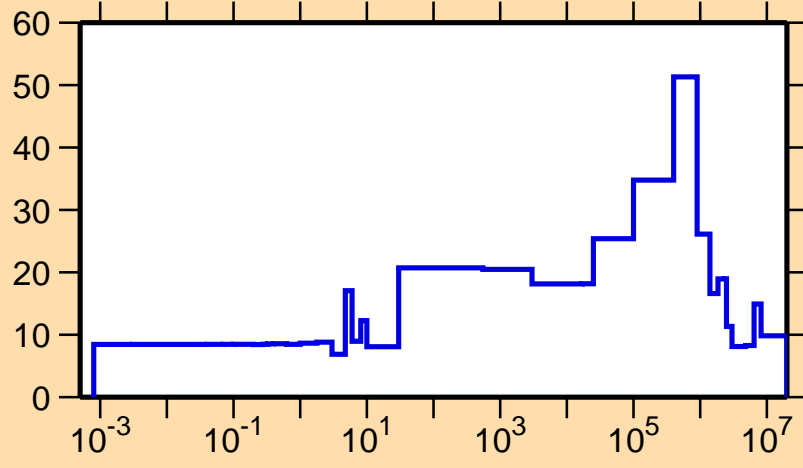
\Delta\sigma/\sigma vs. E for ^{225}\text{Th}(n,el.)
