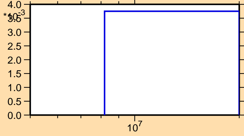
\sigma vs. E for ^{225}\text{Th}(n,3n)
