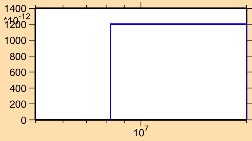
\sigma vs. E for ^{225}\text{Th}(\text{mt } 45)
