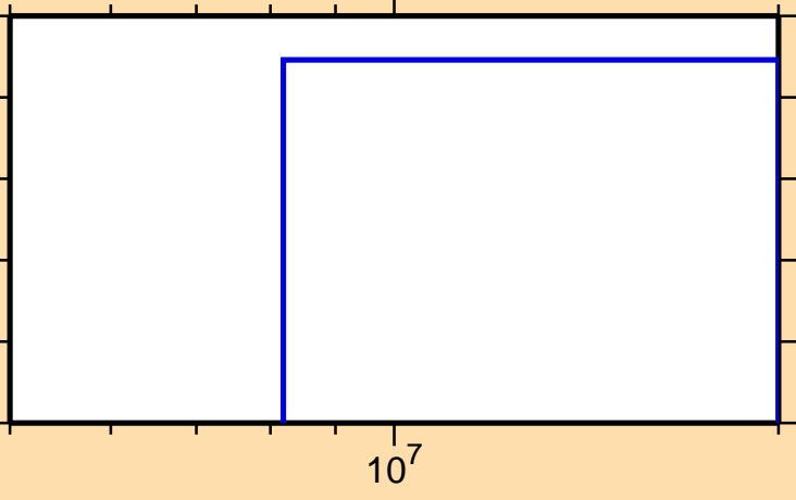
\sigma vs. E for ^{225}\text{Th}(n,3n\alpha)
