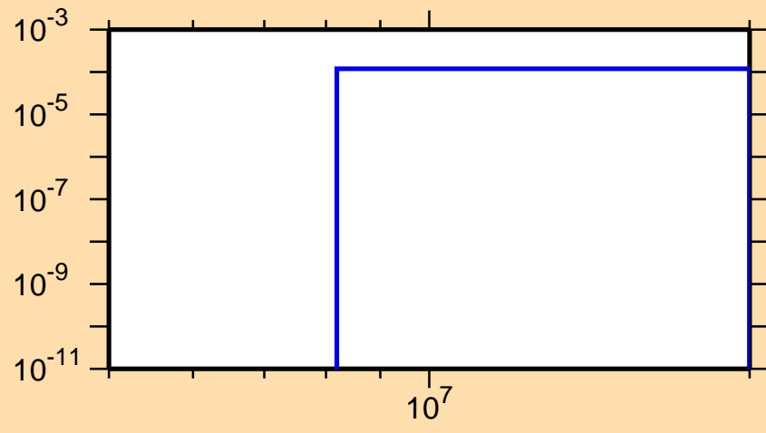
\sigma vs. E for ^{225}\text{Th}(n,t)
