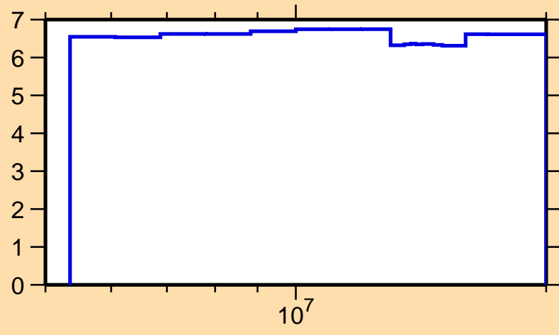
\Delta\sigma/\sigma vs. E for ^{227}\text{Th}(n,\text{nonel.})
