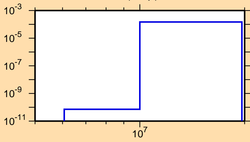
\sigma vs. E for ^{227}\text{Th}(n,np)
