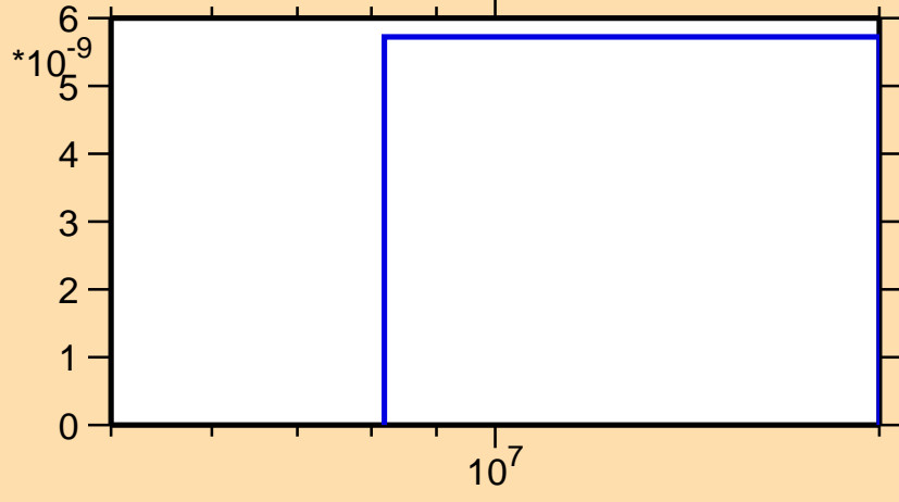
\sigma vs. E for ^{227}\text{Th}(n,nt)
