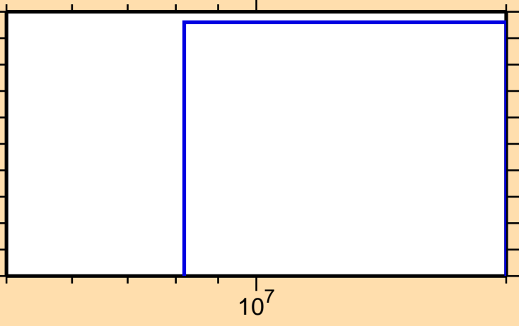
\sigma vs. E for ^{227}\text{Th}(n,3n\alpha)
