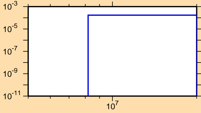
\sigma vs. E for ^{227}\text{Th}(n,d)
