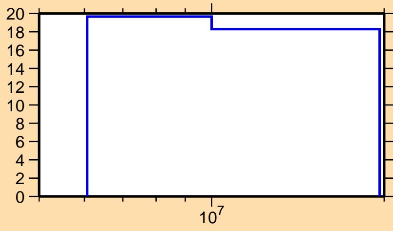
\Delta\sigma/\sigma vs. E for ^{228}\text{Th}(n,2n)
