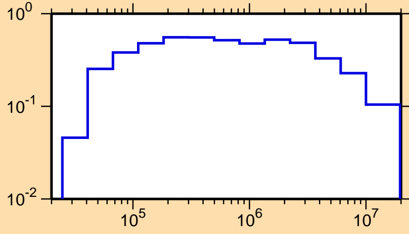
\sigma vs. E for ^{229}\text{Th}(n,n_2)
