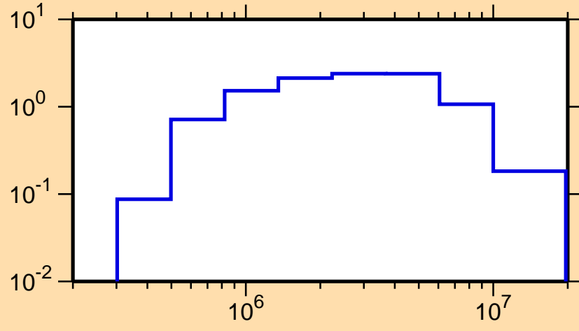
\sigma vs. E for ^{229}\text{Th}(n,n\text{cont.})
