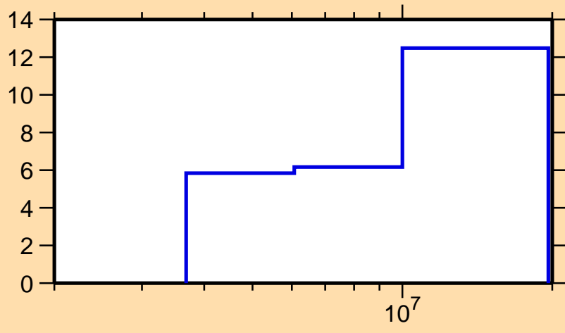
Δσ/σ vs. E for ^{229}\text{Th}(n,2n)
