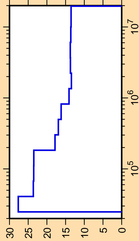
\Delta\sigma/\sigma vs. E for ^{229}\text{Th}(n,n_2)
