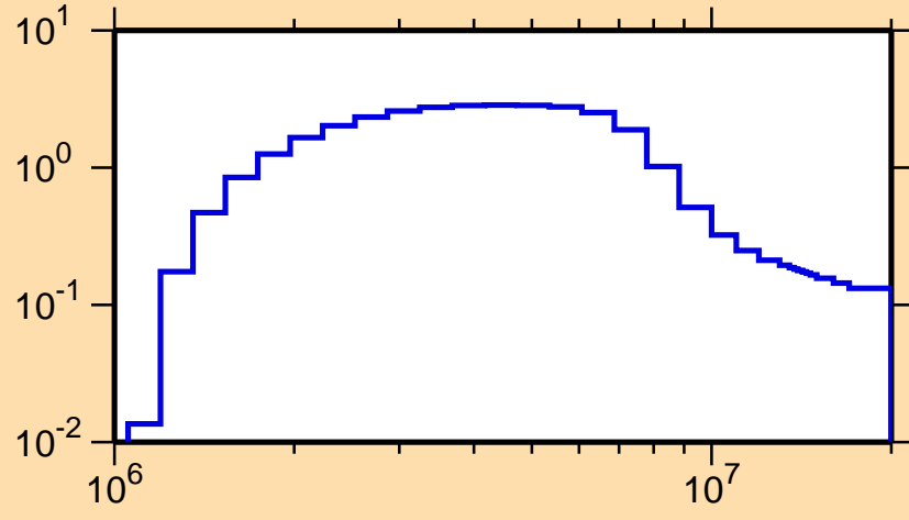
\sigma vs. E for ^{230}\text{Th}(n,n\text{cont.})
