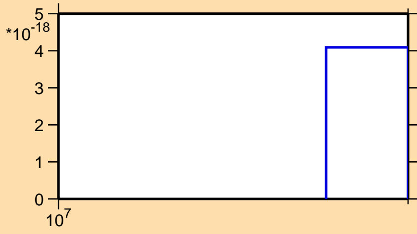
\sigma vs. E for ^{230}\text{Th} (mt 42)
