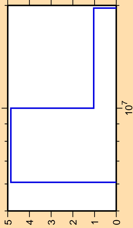
\Delta\sigma/\sigma vs. E for ^{230}\text{Th}(n,\alpha)
