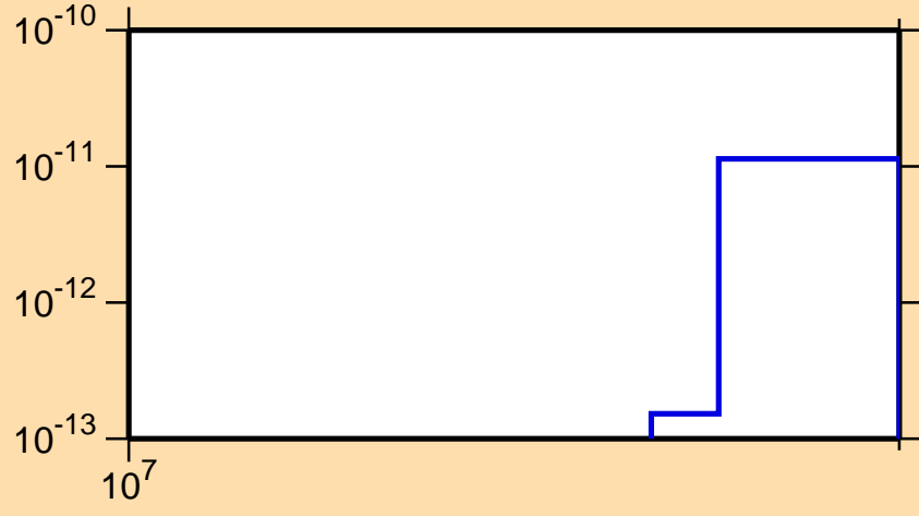
\sigma vs. E for ^{231}\text{Th}(n,3n\alpha)
