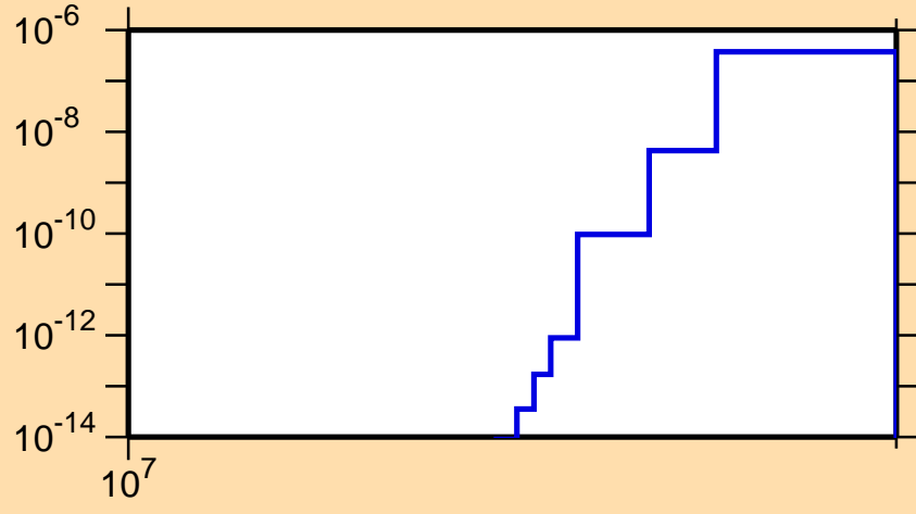
\sigma vs. E for ^{231}\text{Th}(n,nt)
