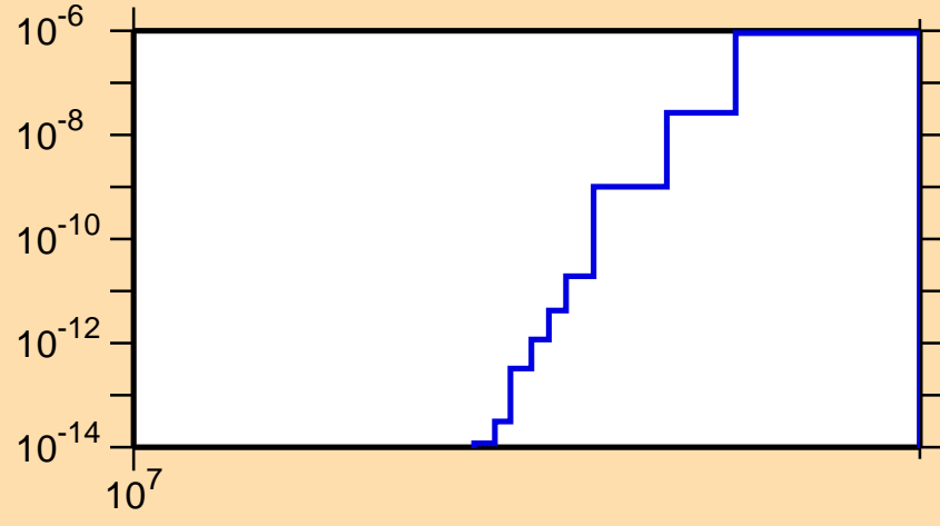
\sigma vs. E for ^{231}\text{Th}(n,\text{nd})
