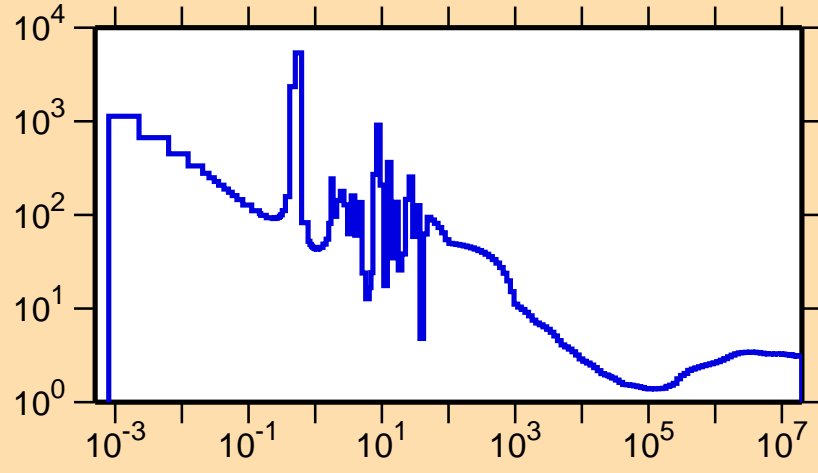
\sigma vs. E for ^{231}\text{Th}(n,\text{nonel.})
