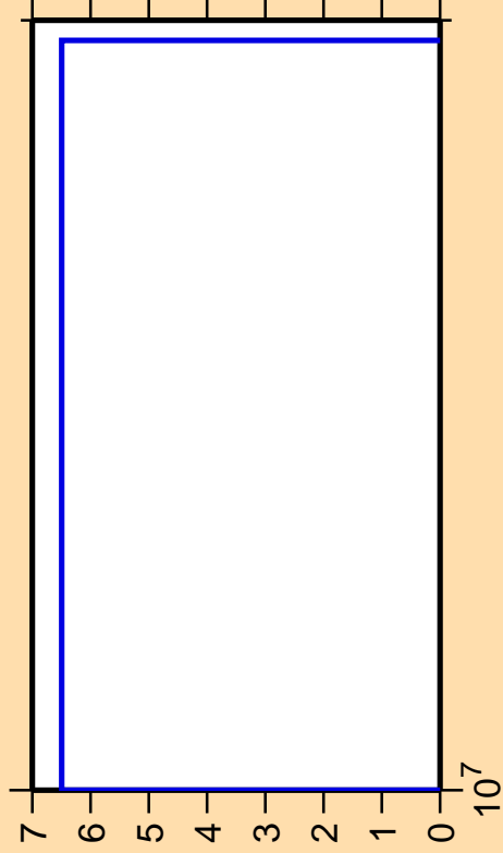
\Delta\sigma/\sigma vs. E for ^{231}\text{Th}(n,\text{nd})
