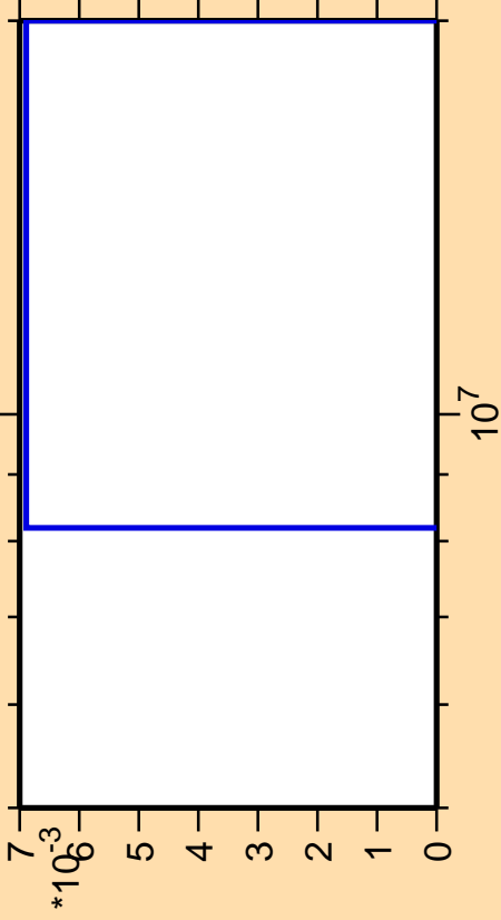
\Delta\sigma/\sigma vs. E for ^{231}\text{Th}(n,\text{He3})
