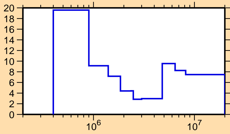
\Delta\sigma/\sigma vs. E for ^{231}\text{Th}(n,n\text{cont.})
