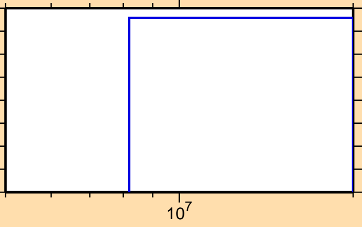
\sigma vs. E for ^{231}\text{Th}(n,\text{He3})
