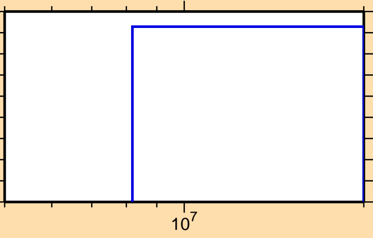
\sigma vs. E for ^{231}\text{Th}(n,t)
