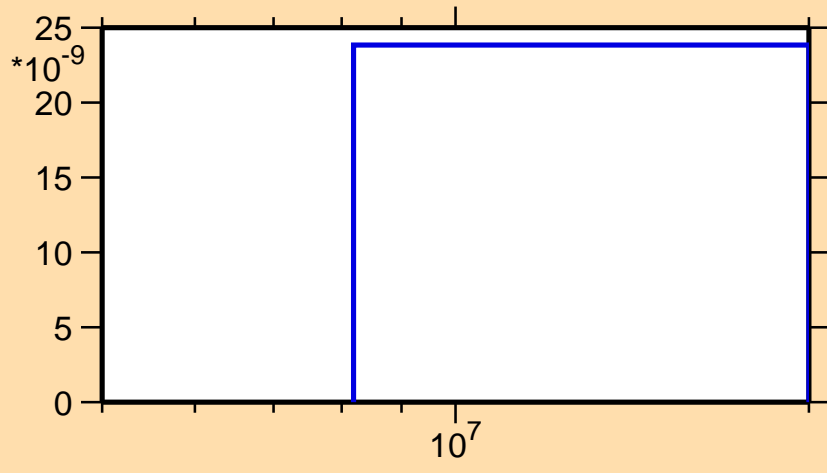
\sigma vs. E for ^{231}\text{Th}(n,2n\alpha)
