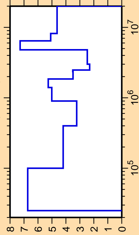
\Delta\sigma/\sigma vs. E for ^{231}\text{Th}(n,\text{inel.})
