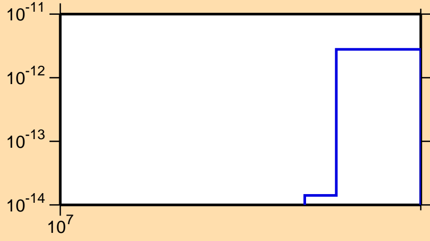
\sigma vs. E for ^{234}\text{Th}(n,3n\alpha)
