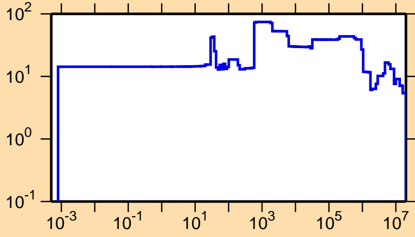
\Delta\sigma/\sigma vs. E for ^{234}\text{Th}(n,el.)
