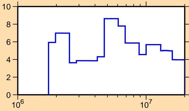
\Delta\sigma/\sigma vs. E for ^{234}\text{Th}(n,\text{tot.})
