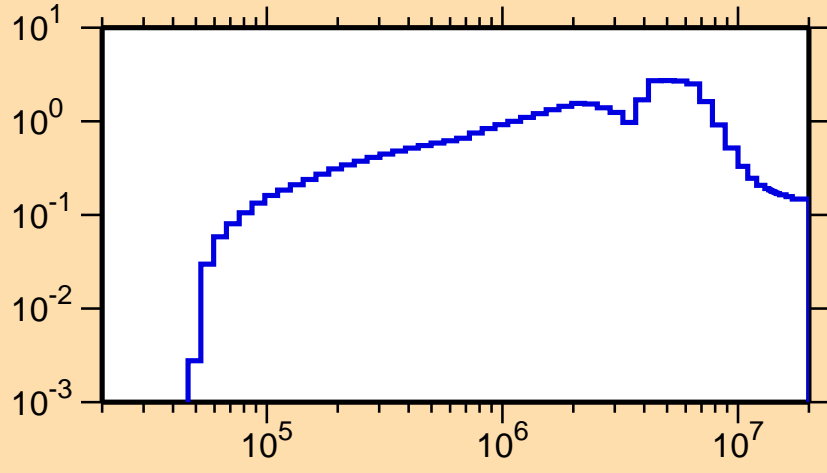
\sigma vs. E for ^{234}\text{Th}(n,\text{inel.})
