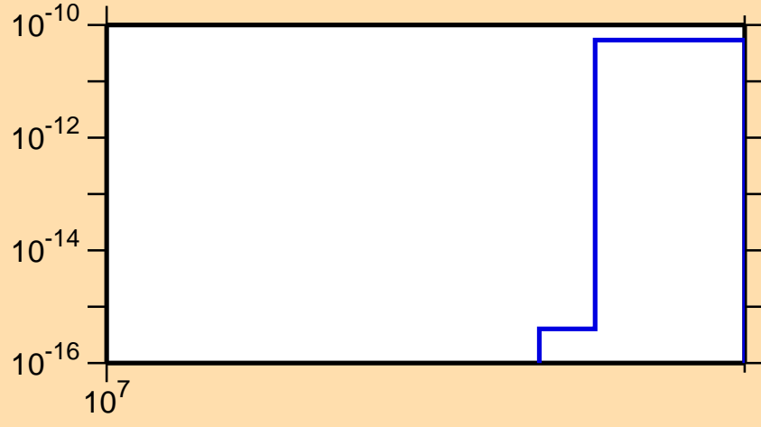
\sigma vs. E for ^{234}\text{Th}(n,2np)
