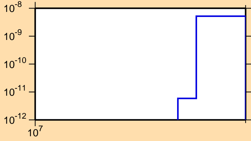
\sigma vs. E for ^{234}\text{Th}(n,\text{nd})
