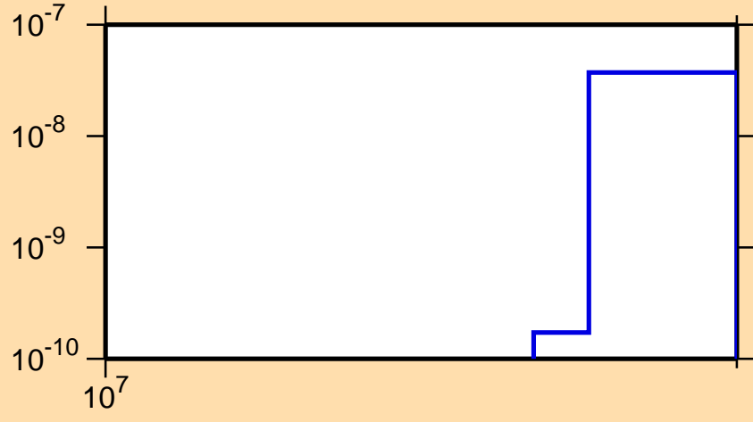
\sigma vs. E for ^{235}\text{Th}(n,2np)
