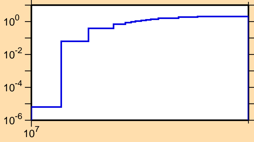
\sigma vs. E for ^{235}\text{Th}(n,3n)
