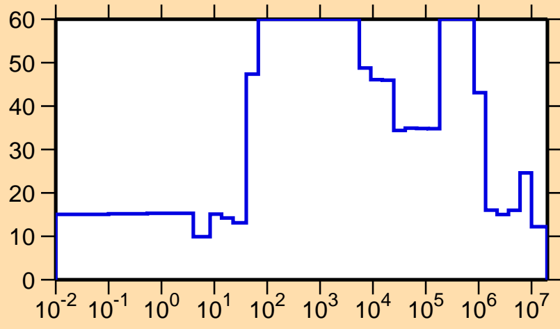
\Delta\sigma/\sigma vs. E for ^{235}\text{Th}(n,el.)
