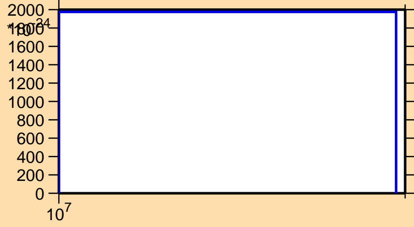
\sigma vs. E for ^{235}\text{Th} (mt 42)
