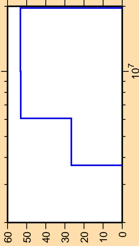
\Delta\sigma/\sigma vs. E for ^{235}\text{Th}(n,n\text{cont.})
