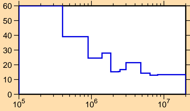
\Delta\sigma/\sigma vs. E for ^{235}\text{Th}(n,\text{nonel.})
