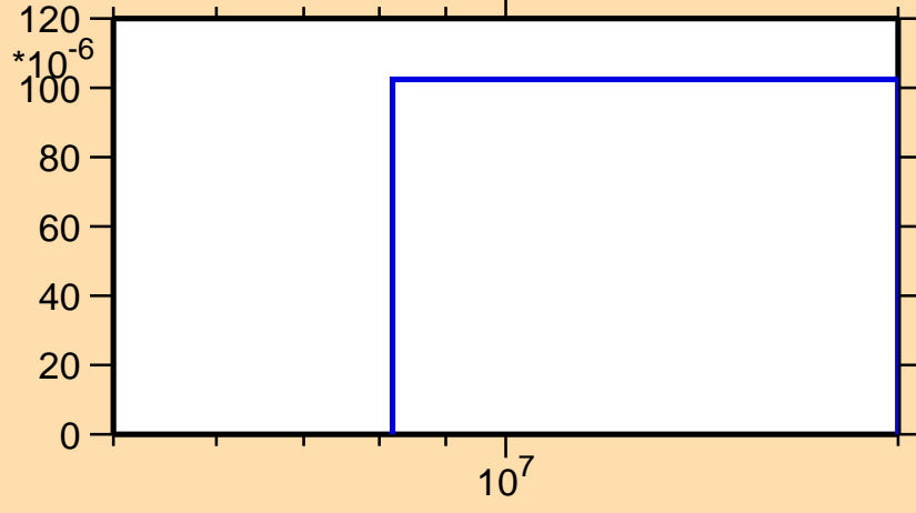
\sigma vs. E for ^{235}\text{Th}(n,t)
