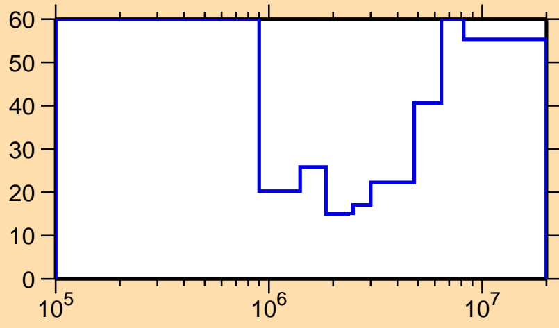
\Delta\sigma/\sigma vs. E for ^{235}\text{Th}(n,n\text{cont.})
