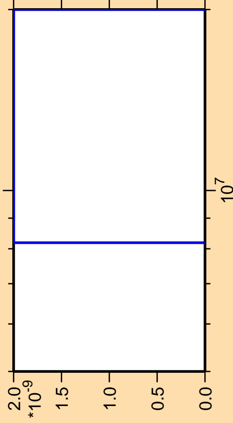
\Delta\sigma/\sigma vs. E for ^{235}\text{Th} (mt 42)
