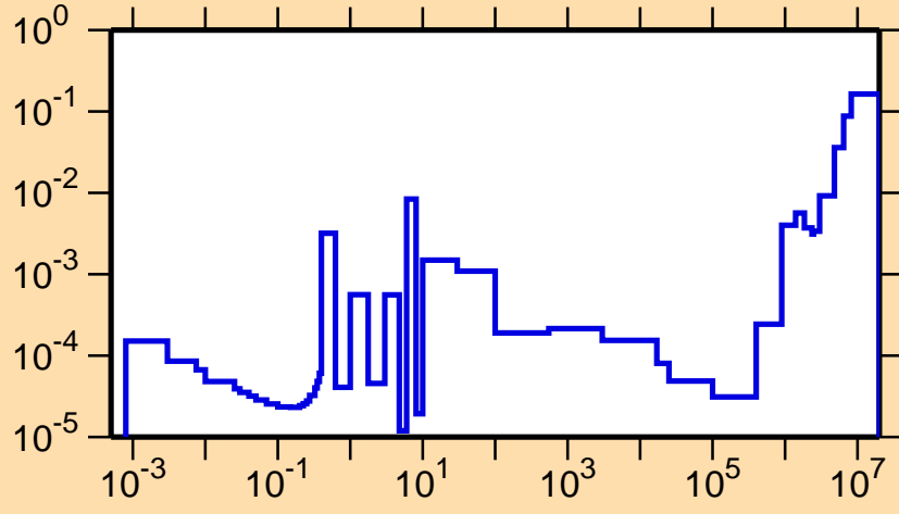
\sigma vs. E for ^{235}\text{Th}(n,f)
