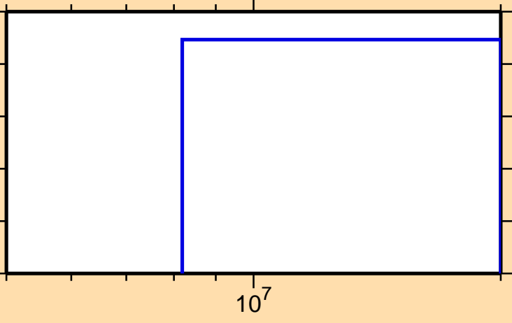
\sigma vs. E for ^{235}\text{Th} (mt 42)
