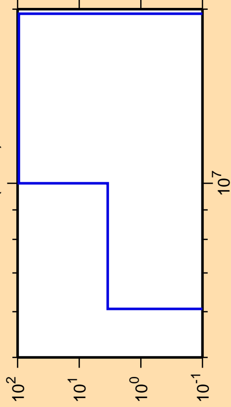
\Delta\sigma/\sigma vs. E for ^{236}\text{Th}(n,n\alpha)
