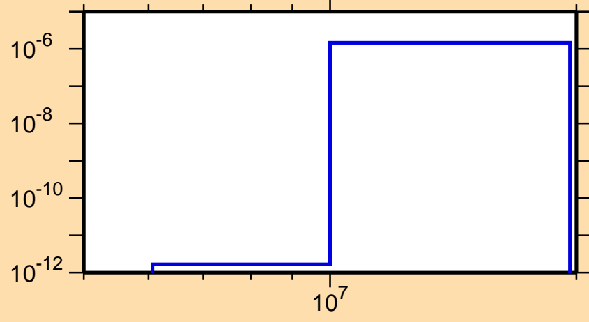
\sigma vs. E for ^{236}\text{Th}(n,n\alpha)
