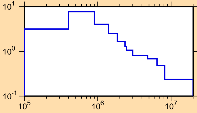
\sigma vs. E for ^{236}\text{Th}(n,n_1)
