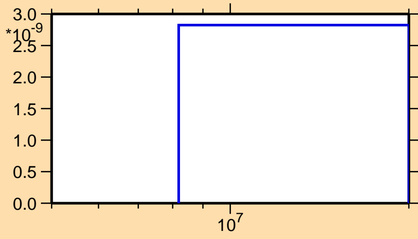
\sigma vs. E for ^{236}\text{Th}(n,nt)
