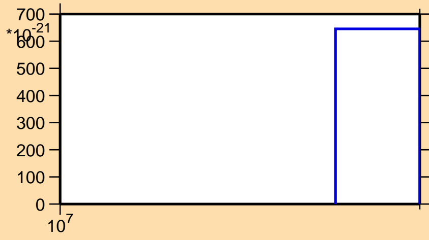
\sigma vs. E for ^{237}\text{Th} (mt 42)
