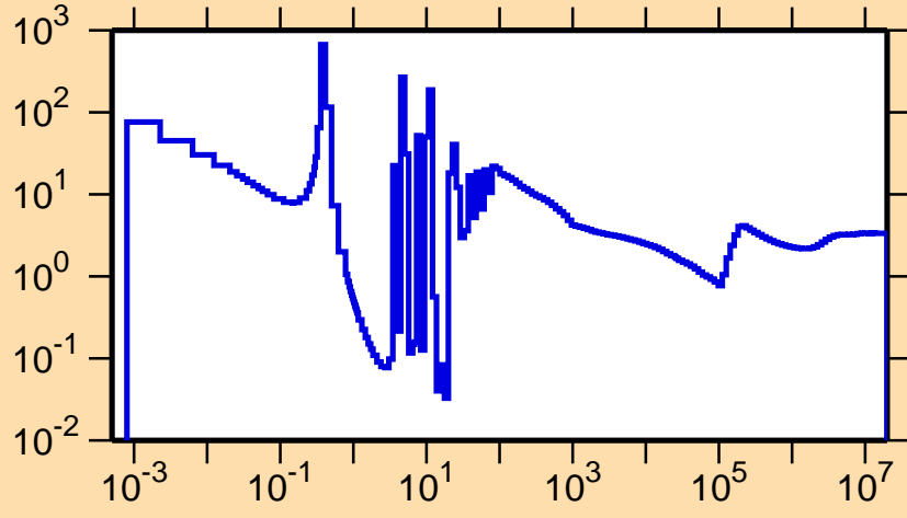
\sigma vs. E for ^{237}\text{Th}(n,\text{nonel.})
