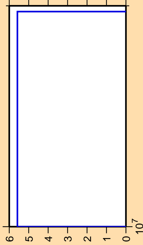
\Delta\sigma/\sigma vs. E for ^{237}\text{Th}(n,2np)
