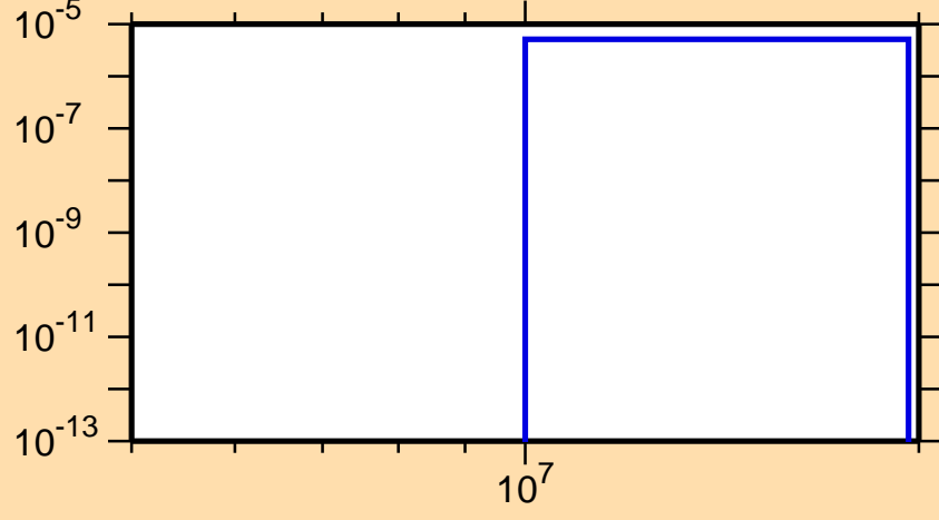
\sigma vs. E for ^{237}\text{Th}(n,np)
