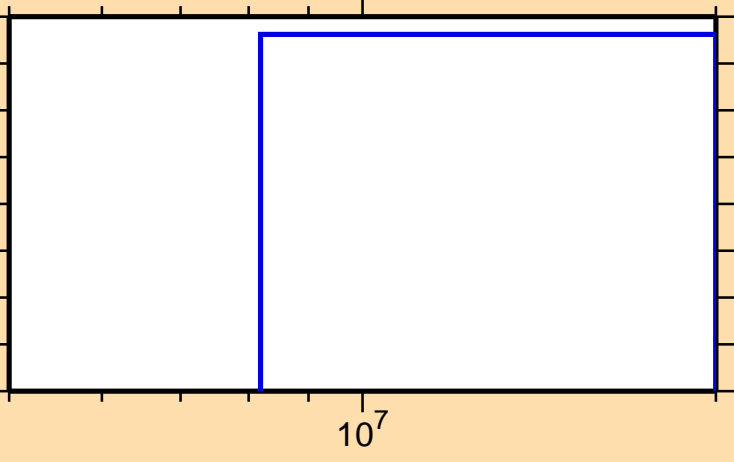
\sigma vs. E for ^{237}\text{Th}(n,d)
