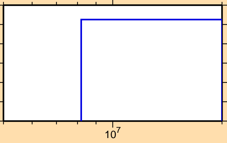
\sigma vs. E for ^{237}\text{Th} (mt 42)
