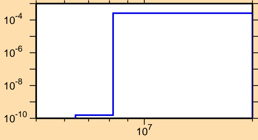
\sigma vs. E for ^{237}\text{Th}(n,p)
