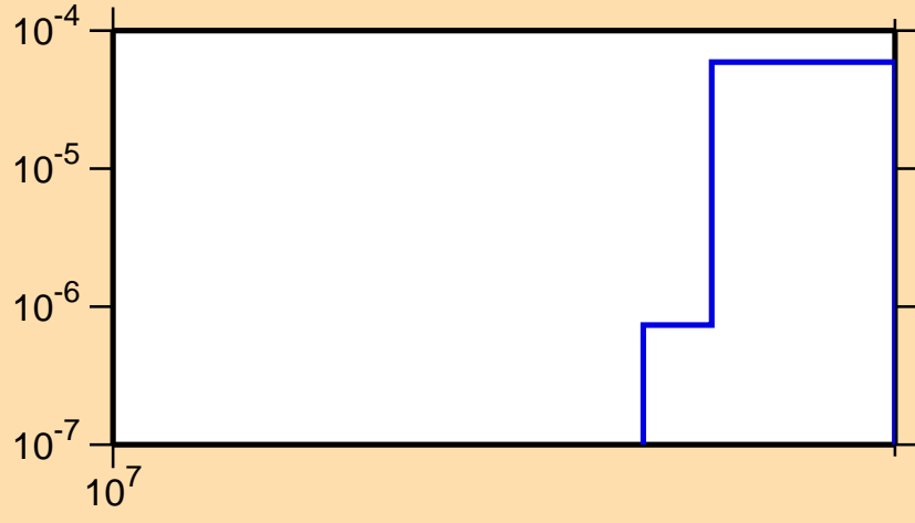
\sigma vs. E for ^{238}\text{Th}(n,\text{nd})
