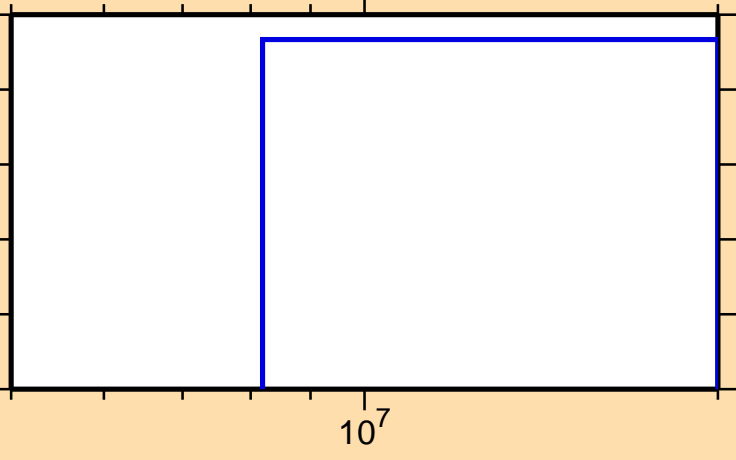
\sigma vs. E for ^{238}\text{Th}(n,nt)
