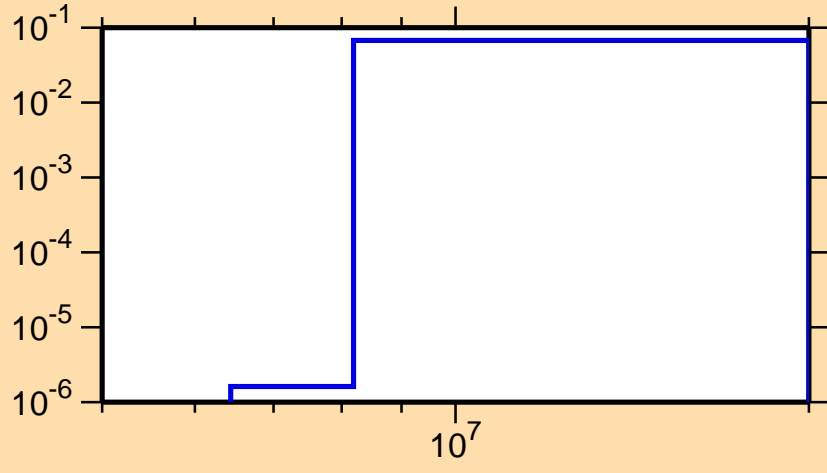
\sigma vs. E for ^{238}\text{Th}(n,\alpha)
