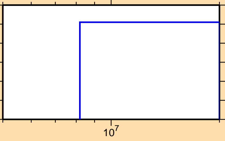
\sigma vs. E for ^{238}\text{Th}(n,\text{nd})
