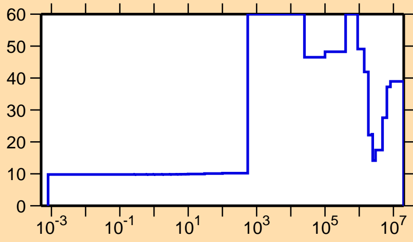
\Delta\sigma/\sigma vs. E for ^{238}\text{Th}(n,el.)
