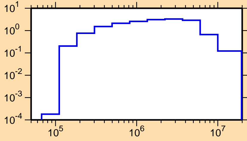
\sigma vs. E for ^{239}\text{Th}(n,n\text{cont.})
