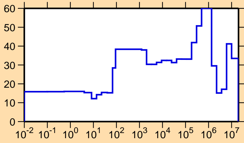
\Delta\sigma/\sigma vs. E for ^{239}\text{Th}(n,el.)
