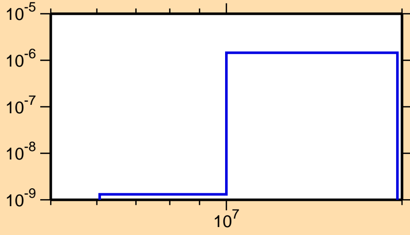
\sigma vs. E for ^{239}\text{Th}(n,n\alpha)
