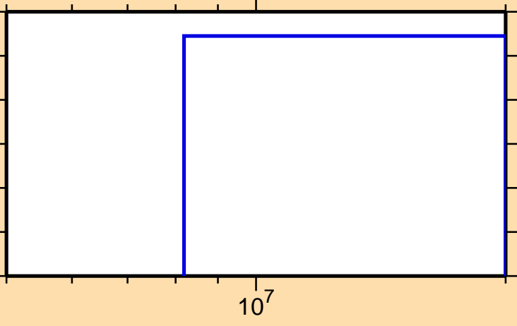
\sigma vs. E for ^{239}\text{Th}(n,nt)
