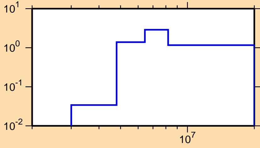
\sigma vs. E for ^{239}\text{Th}(n,2n)
