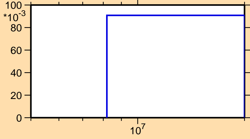
\sigma vs. E for ^{239}\text{Th}(n,3n)
