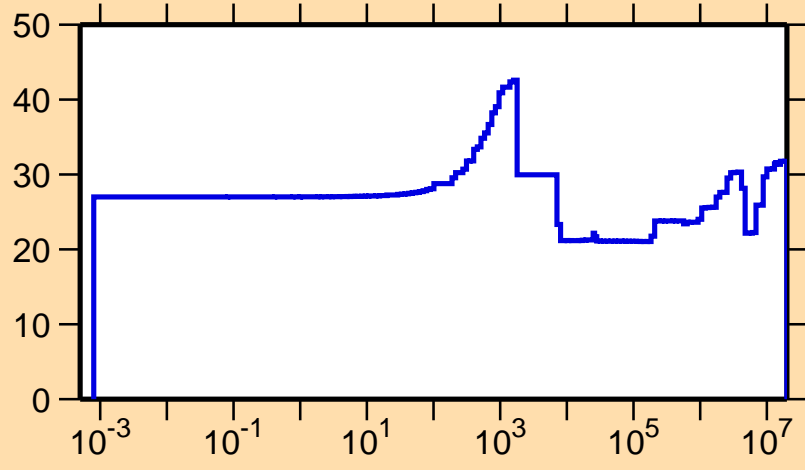
\Delta\sigma/\sigma vs. E for ^{44}\text{Ti}(n,\gamma)
