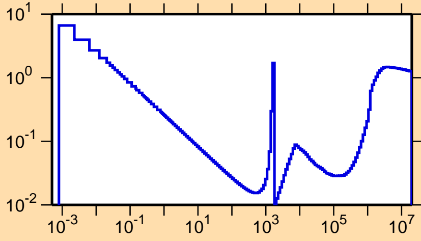
\sigma vs. E for ^{44}\text{Ti}(n,\text{nonel.})
