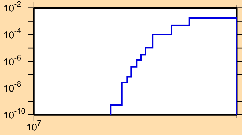
\sigma vs. E for ^{44}\text{Ti}(n,\text{pd})
