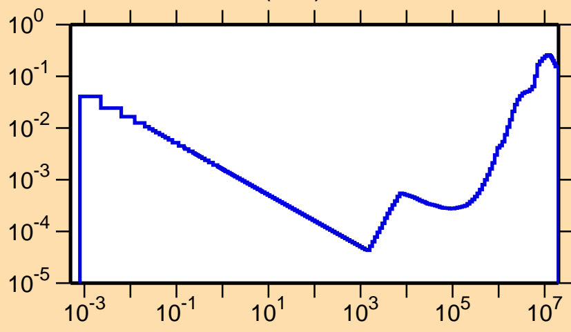
\sigma vs. E for ^{44}\text{Ti}(n,\alpha)
