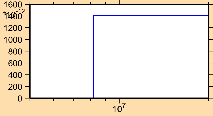
\sigma vs. E for ^{44}\text{Ti}(\text{mt } 45)
