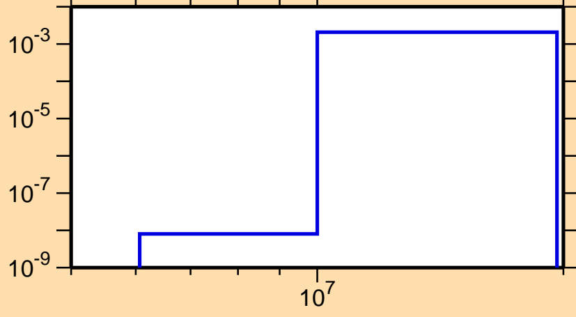
\sigma vs. E for ^{45}\text{Ti}(n,p\alpha)
