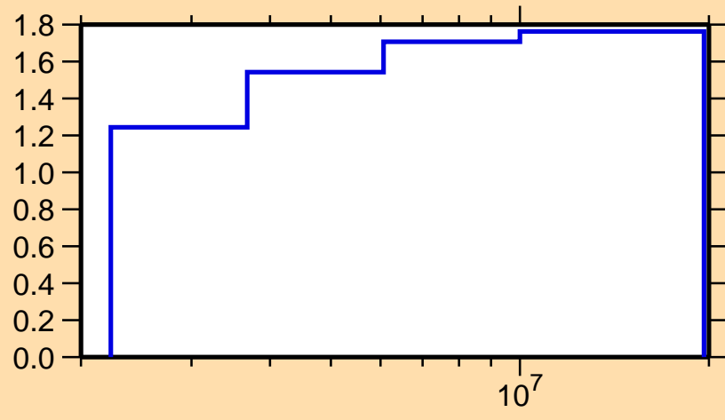
\Delta\sigma/\sigma vs. E for ^{45}\text{Ti}(n,n\text{onel.})
