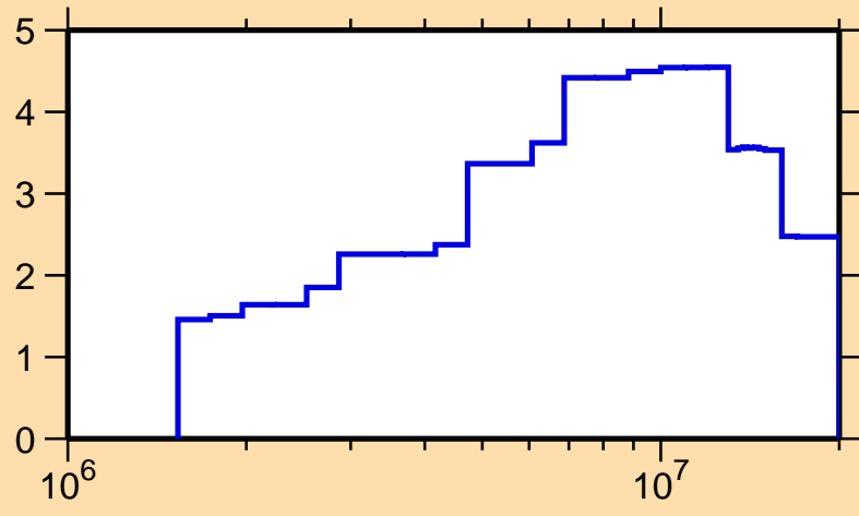
\Delta\sigma/\sigma vs. E for ^{46}\text{Ti}(n,el.)
