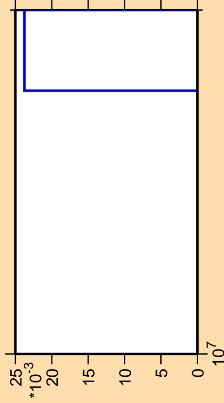
\Delta\sigma/\sigma vs. E for ^{46}\text{Ti}(n,\text{nd})
