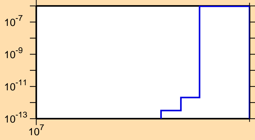
\sigma vs. E for ^{46}\text{Ti}(n,pd)
