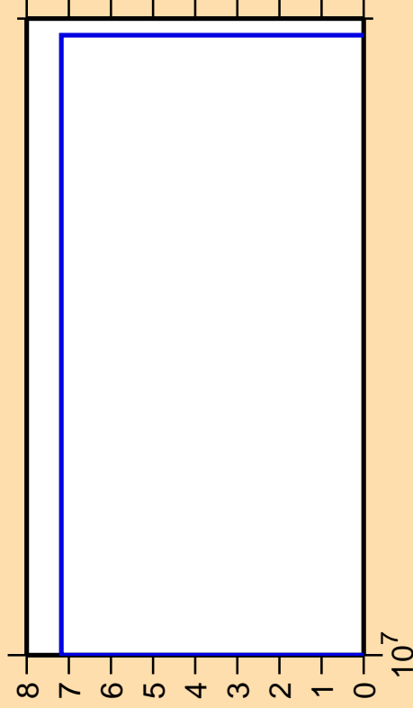
\Delta\sigma/\sigma vs. E for ^{46}\text{Ti}(n,np)
