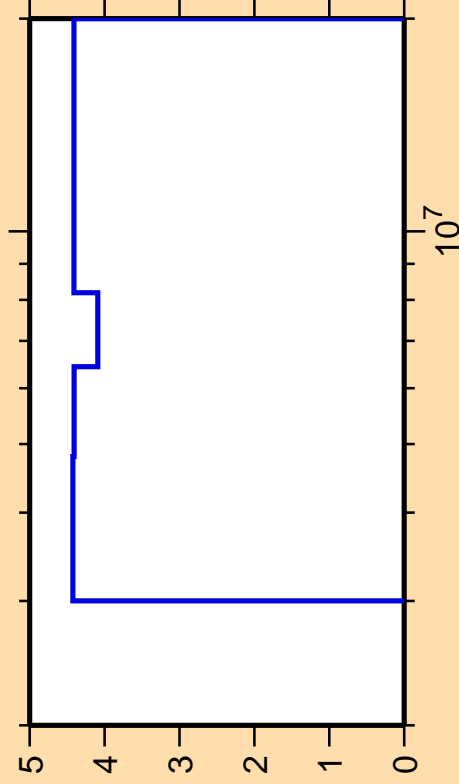
\Delta\sigma/\sigma vs. E for ^{46}\text{Ti}(n,n\text{cont.})
