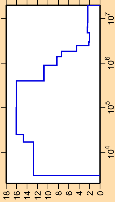
\Delta\sigma/\sigma vs. E for ^{46}\text{Ti}(n,\text{nonel.})
