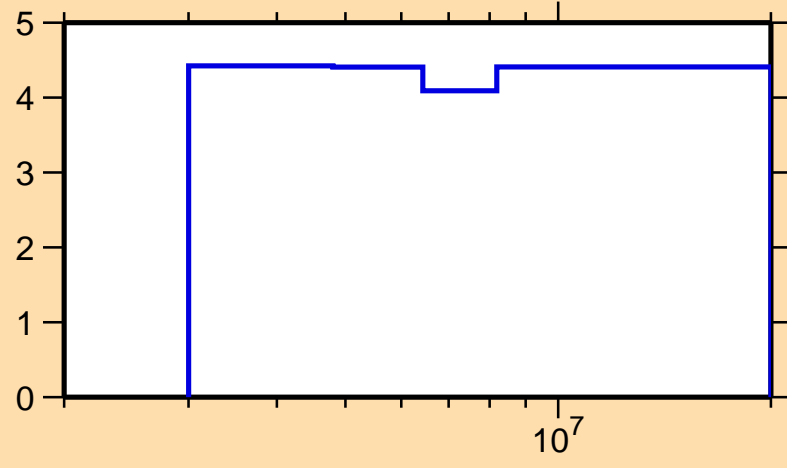
\Delta\sigma/\sigma vs. E for ^{46}\text{Ti}(n,n\text{cont.})
