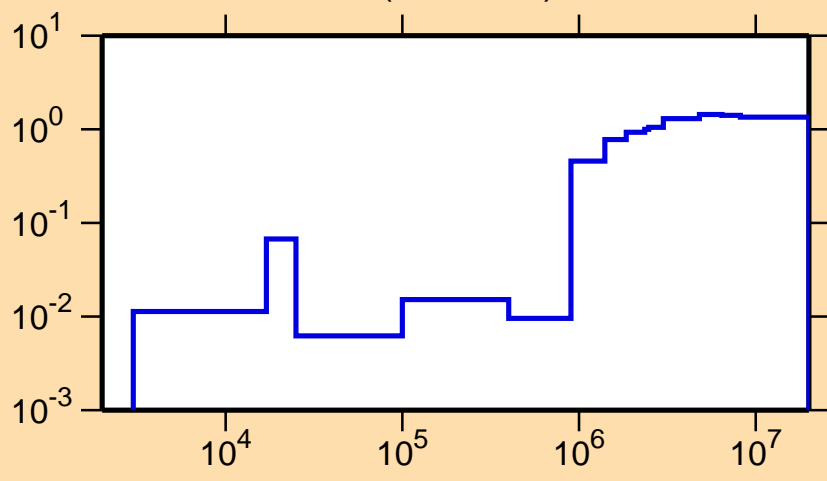
\sigma vs. E for ^{46}\text{Ti}(n,\text{nonel.})
