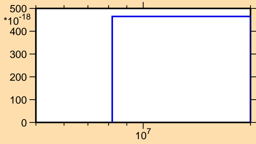
\sigma vs. E for ^{46}\text{Ti}(n,nd)
