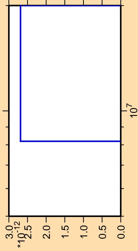
\Delta\sigma/\sigma vs. E for ^{46}\text{Ti} (mt 45)
