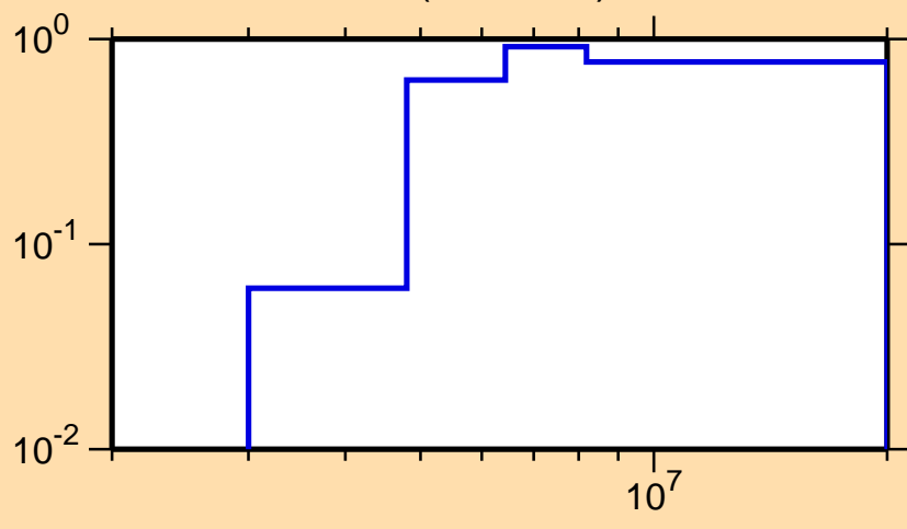
\sigma vs. E for ^{46}\text{Ti}(n,n\text{cont.})
