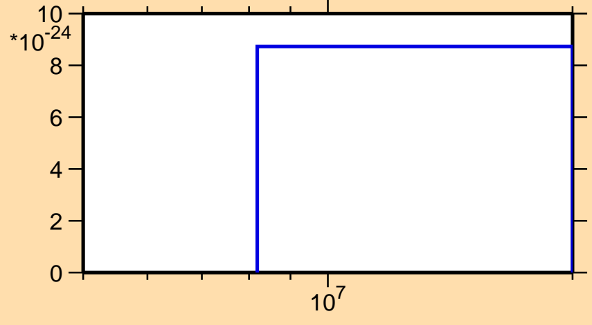
\sigma vs. E for ^{46}\text{Ti} (mt 45)
