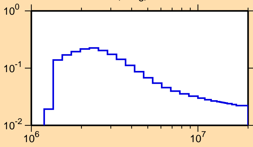
\sigma vs. E for ^{47}\text{Ti}(n,n_3)
