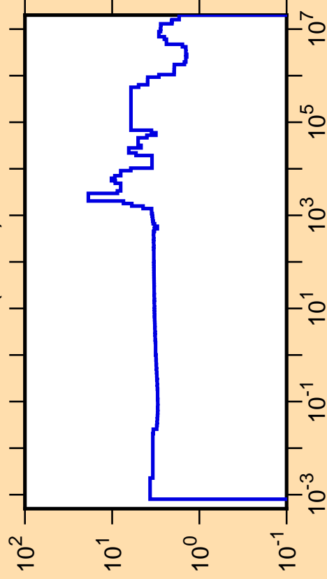
\Delta\sigma/\sigma vs. E for ^{47}\text{Ti}(n,\text{tot.})
