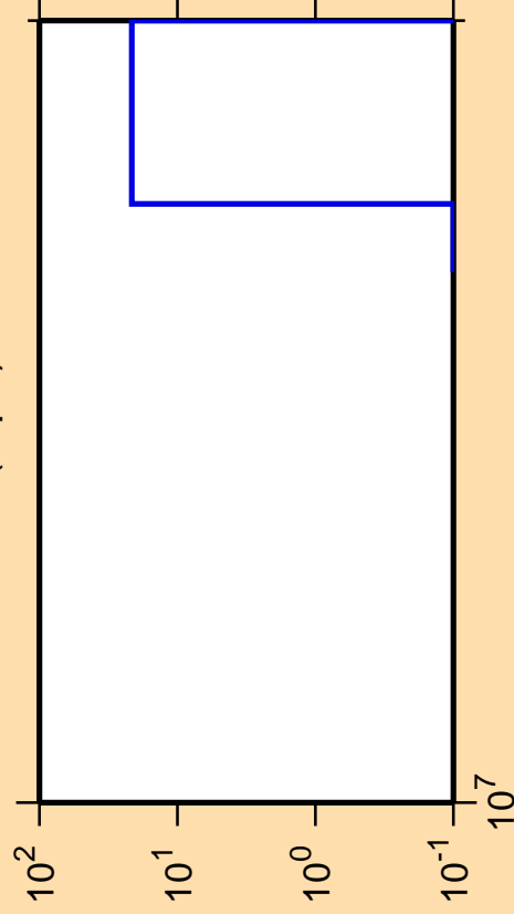
\Delta\sigma/\sigma vs. E for ^{47}\text{Ti}(n,pd)
