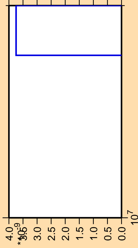
\Delta\sigma/\sigma vs. E for ^{47}\text{Ti} (mt 34)
