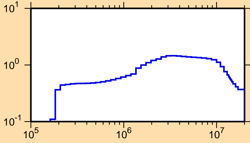
\sigma vs. E for ^{47}\text{Ti}(n,\text{inel.})
