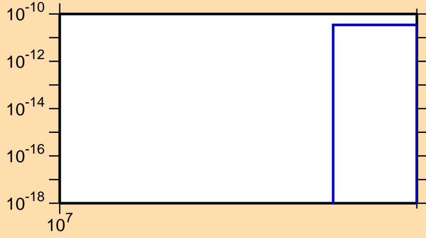
\sigma vs. E for ^{47}\text{Ti}(n,pd)
