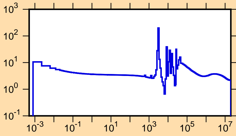
\sigma vs. E for ^{47}\text{Ti}(n,\text{tot.})
