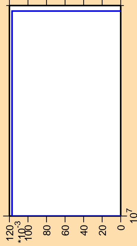
\Delta\sigma/\sigma vs. E for ^{47}\text{Ti}(n,\text{pd})
