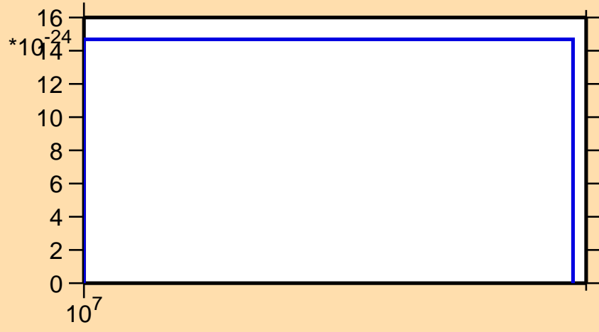
\sigma vs. E for ^{47}\text{Ti} (mt 34)
