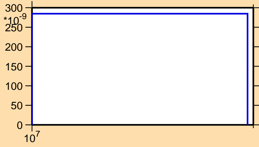
\sigma vs. E for ^{47}\text{Ti}(n,\text{He}3)
