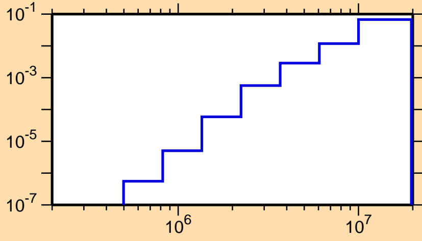
\sigma vs. E for ^{47}\text{Ti}(n,\alpha)
