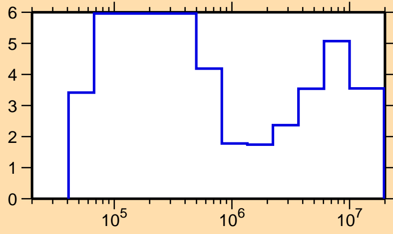
\Delta\sigma/\sigma vs. E for ^{47}\text{Ti}(n,el.)
