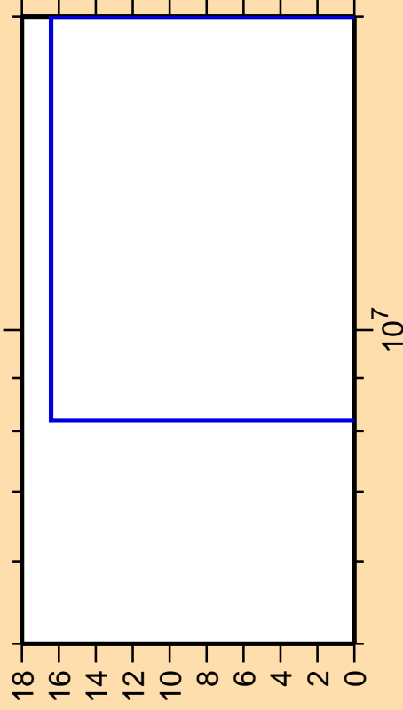
\Delta\sigma/\sigma vs. E for ^{47}\text{Ti}(n,n_1)
