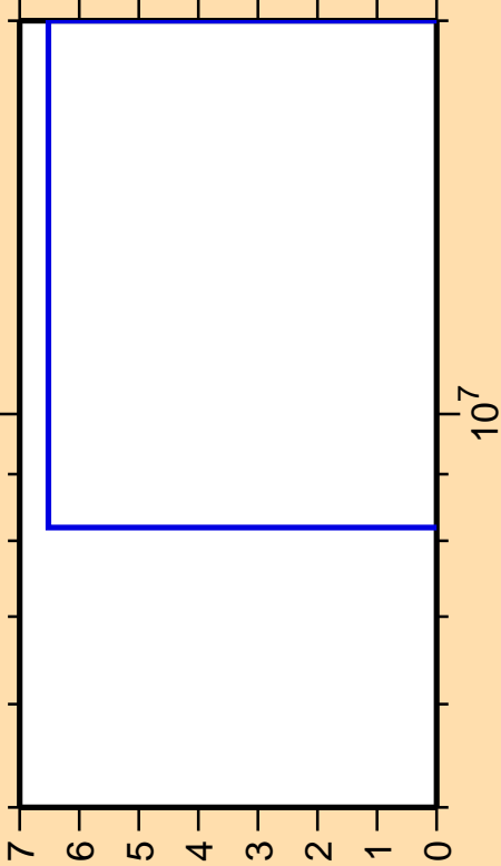
\Delta\sigma/\sigma vs. E for ^{47}\text{Ti}(n,2n)
