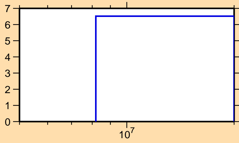
\Delta\sigma/\sigma vs. E for ^{47}\text{Ti}(n,2n)
