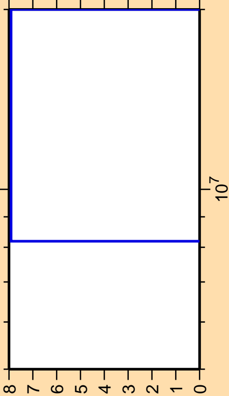
\Delta\sigma/\sigma vs. E for ^{47}\text{Ti}(n,p)
