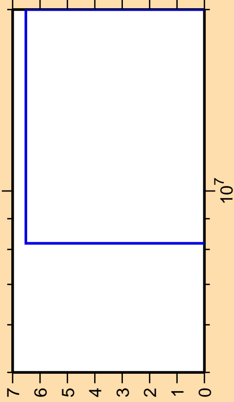
\Delta\sigma/\sigma vs. E for ^{47}\text{Ti}(n,2n)
