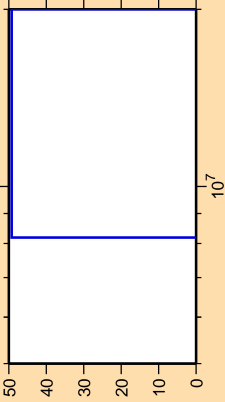
\Delta\sigma/\sigma vs. E for ^{47}\text{Ti}(n,d)
