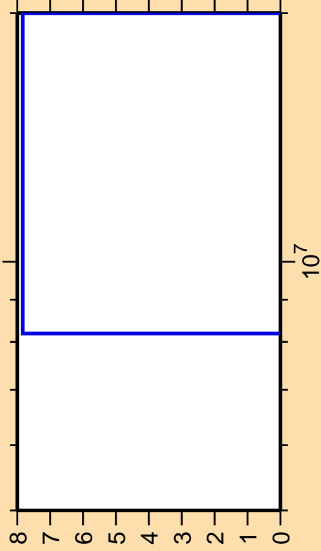
\Delta\sigma/\sigma vs. E for ^{47}\text{Ti}(n,n\text{cont.})
