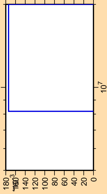
\Delta\sigma/\sigma vs. E for ^{47}\text{Ti}(n,pd)
