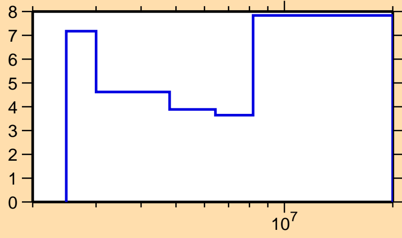
\Delta\sigma/\sigma vs. E for ^{47}\text{Ti}(n,n\text{cont.})
