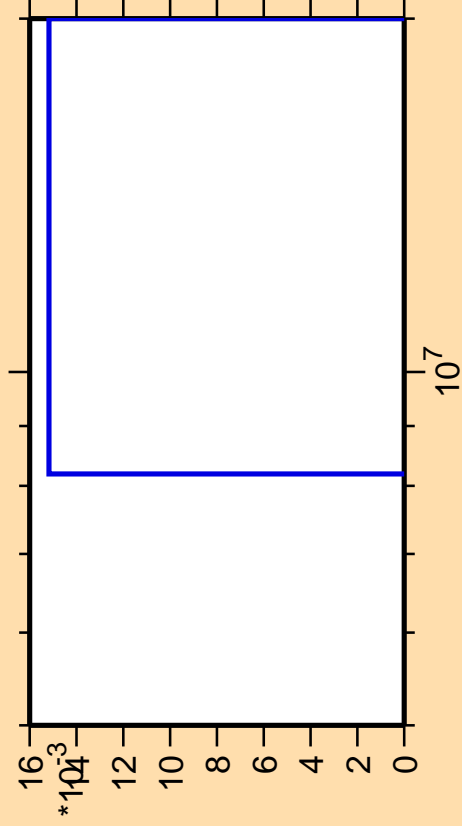
\Delta\sigma/\sigma vs. E for ^{48}\text{Ti}(n,p\alpha)
