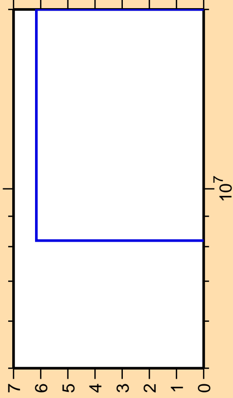
\Delta\sigma/\sigma vs. E for ^{48}\text{Ti}(n,n\text{cont.})
