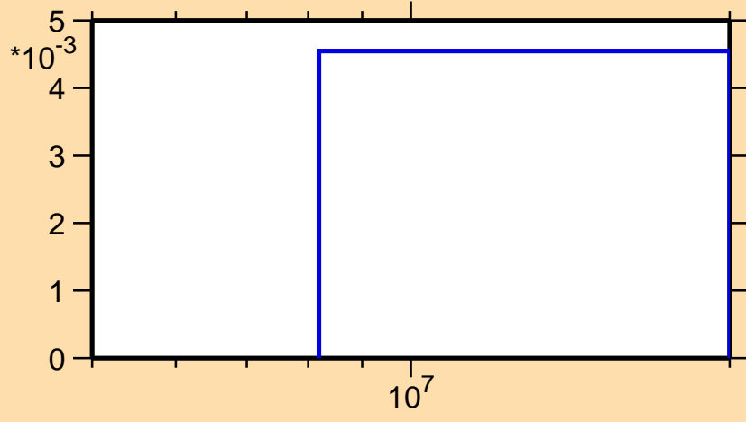
\sigma vs. E for ^{48}\text{Ti}(n,np)
