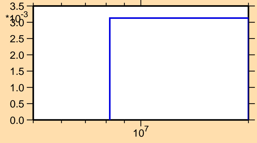
\sigma vs. E for ^{48}\text{Ti}(n,d)
