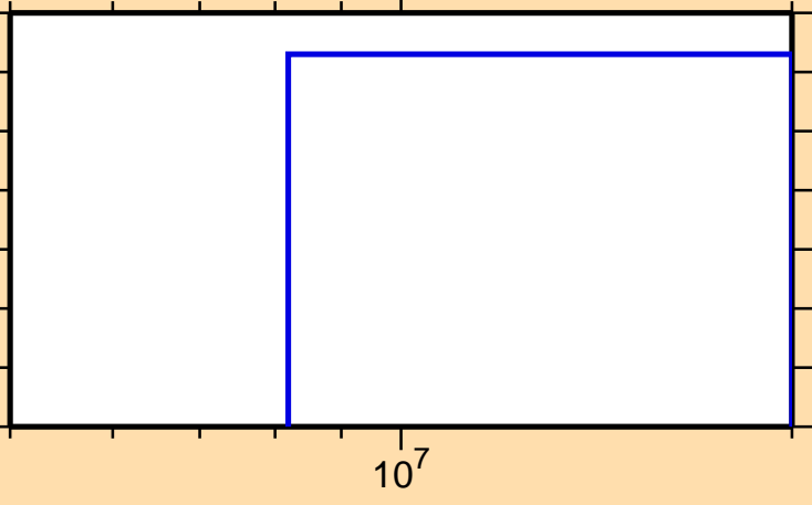
\sigma vs. E for ^{48}\text{Ti}(n,p\alpha)
