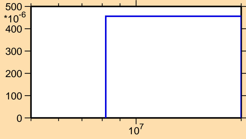
\sigma vs. E for ^{48}\text{Ti}(n,n\alpha)
