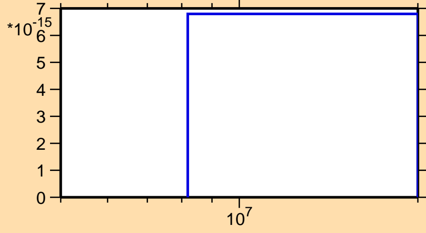
\sigma vs. E for ^{48}\text{Ti}(n,pd)
