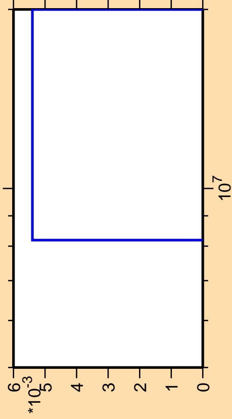
\Delta\sigma/\sigma vs. E for ^{48}\text{Ti}(n,pd)
