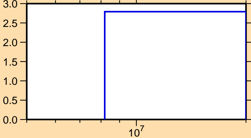
\Delta\sigma/\sigma vs. E for ^{48}\text{Ti}(n,\text{nonel.})
