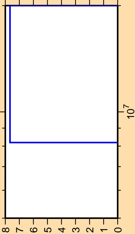
\Delta\sigma/\sigma vs. E for ^{48}\text{Ti}(n,2n)
