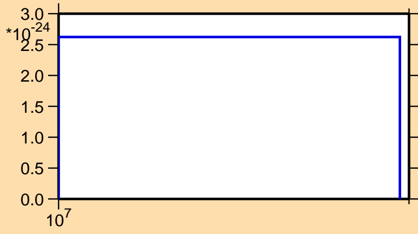
\sigma vs. E for ^{48}\text{Ti} (mt 45)
