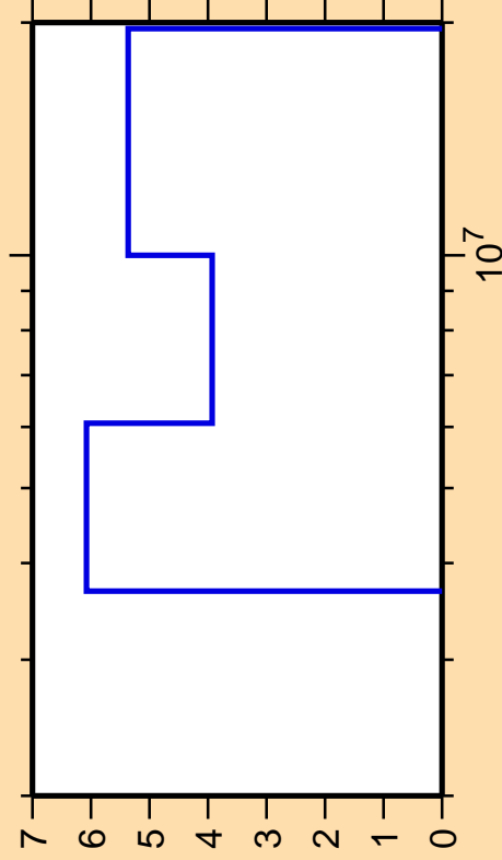
\Delta\sigma/\sigma vs. E for ^{49}\text{Ti}(n,\text{ncont.})
