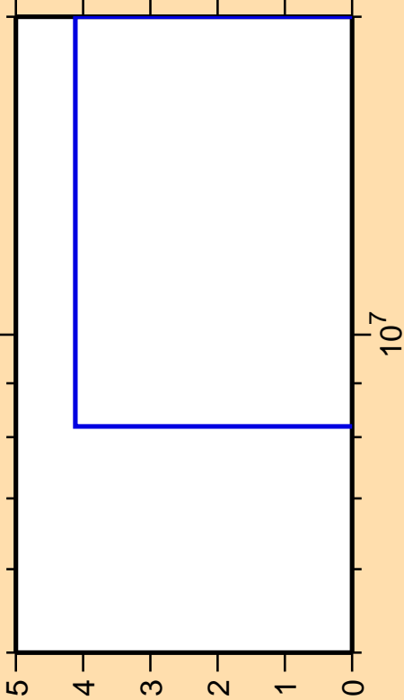
\Delta\sigma/\sigma vs. E for ^{49}\text{Ti}(n,2n)
