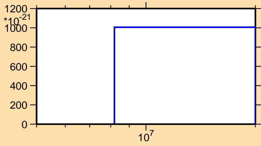
\sigma vs. E for ^{49}\text{Ti}(n,\text{pd})
