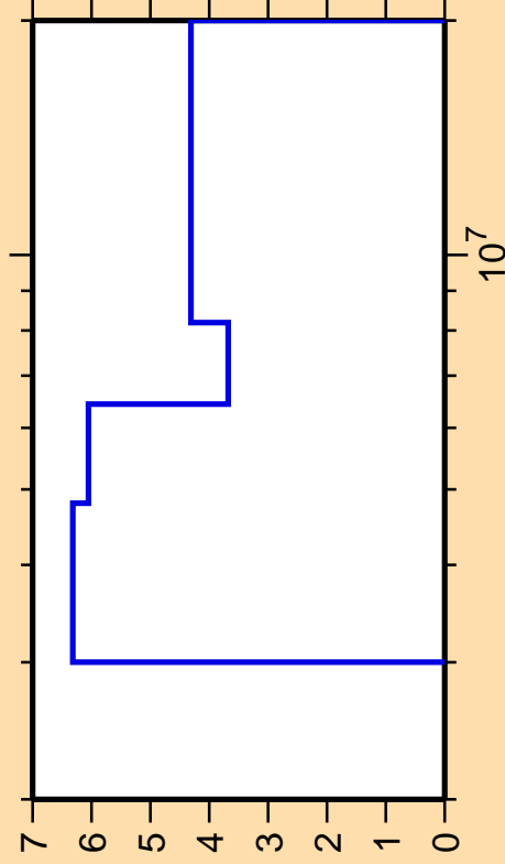
\Delta\sigma/\sigma vs. E for ^{49}\text{Ti}(n,n_{\text{cont}})
