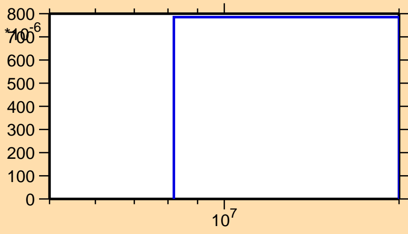
\sigma vs. E for ^{49}\text{Ti}(n,d)
