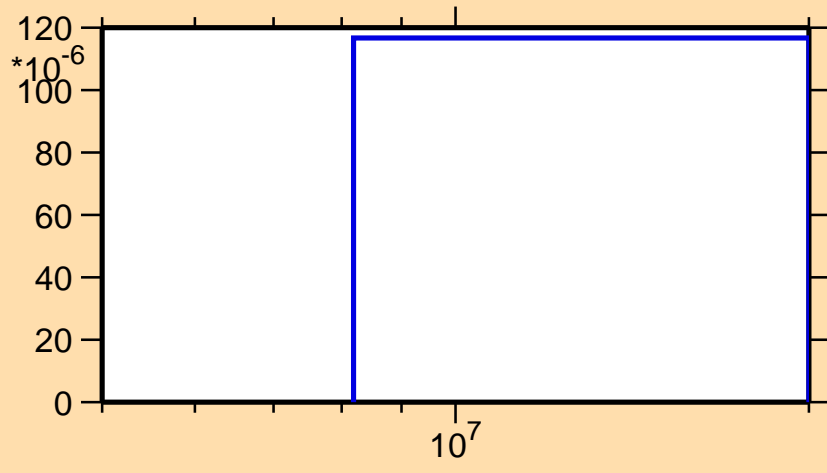
\sigma vs. E for ^{49}\text{Ti}(n,n\alpha)
