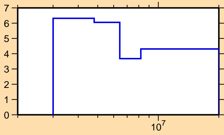
\Delta\sigma/\sigma vs. E for ^{49}\text{Ti}(n,n\text{cont.})
