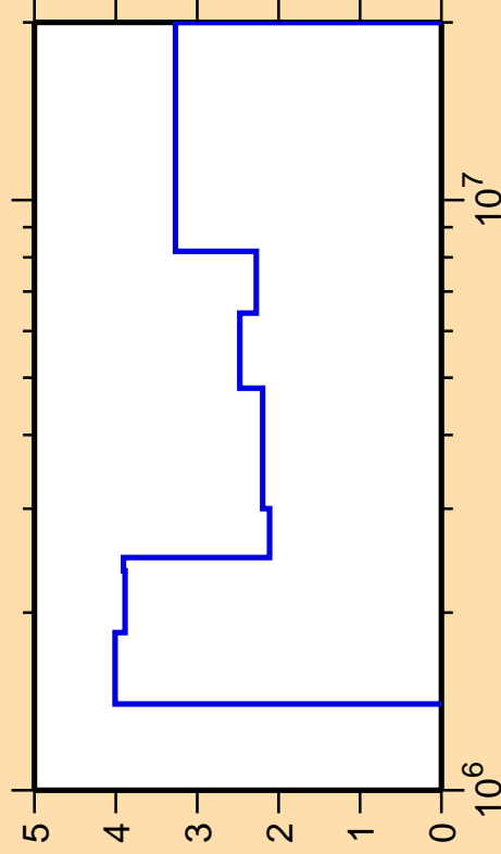
\Delta\sigma/\sigma vs. E for ^{49}\text{Ti}(n,\text{inel.})
