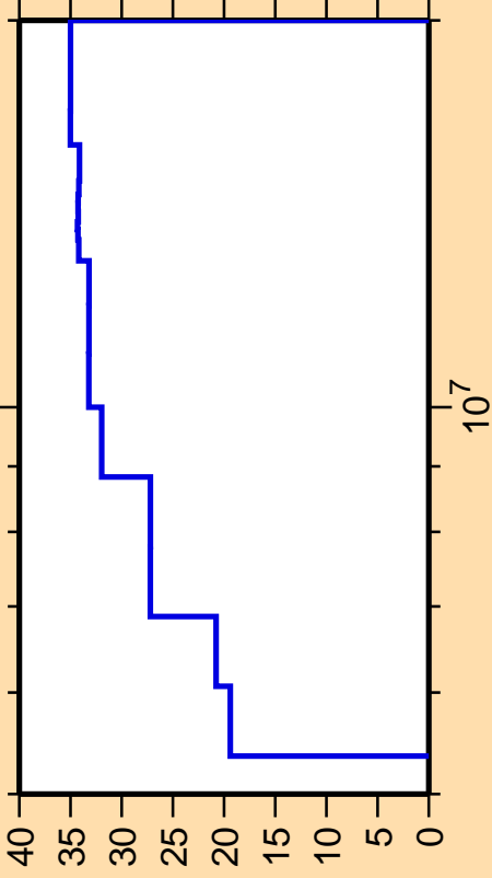
\Delta\sigma/\sigma vs. E for ^{50}\text{Ti}(n,\gamma)
