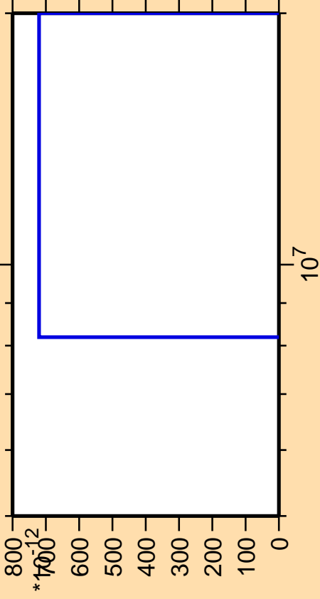
\Delta\sigma/\sigma vs. E for ^{50}\text{Ti}(n,p\alpha)
