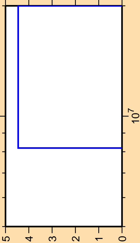
\Delta\sigma/\sigma vs. E for ^{50}\text{Ti}(n,2n)
