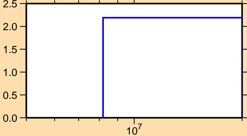
\Delta\sigma/\sigma vs. E for ^{50}\text{Ti}(n,\text{nonel.})
