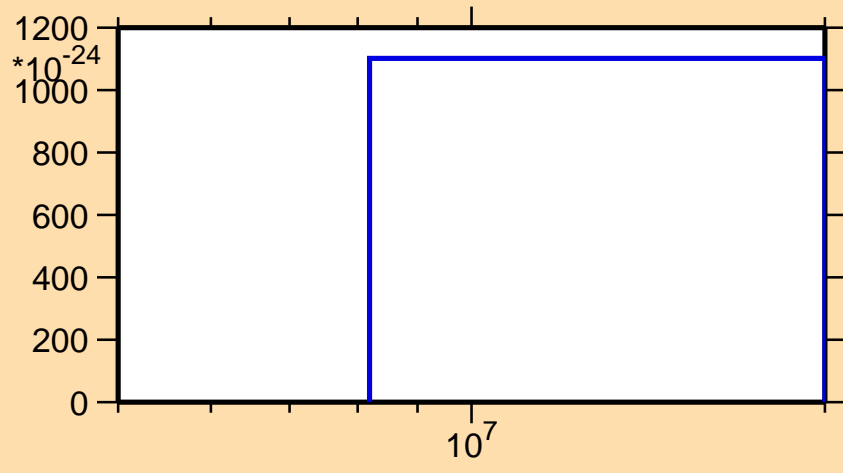
\sigma vs. E for ^{50}\text{Ti}(n,p\alpha)
