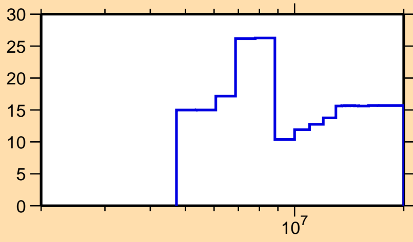
\Delta\sigma/\sigma vs. E for ^{51}\text{Ti}(n,n_1)
