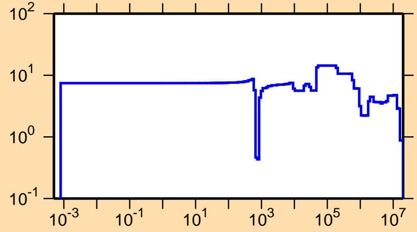
\Delta\sigma/\sigma vs. E for ^{51}\text{Ti}(n,\text{el.})
