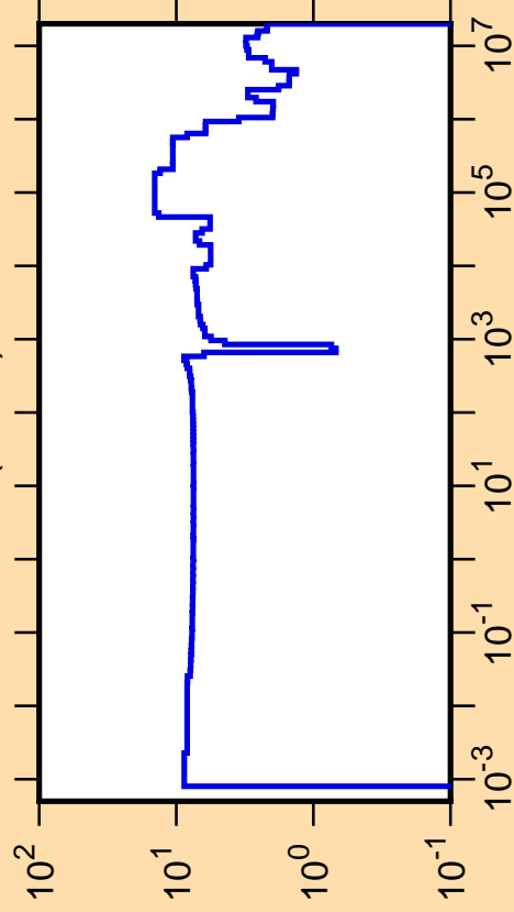
\Delta\sigma/\sigma vs. E for ^{51}\text{Ti}(n,\text{tot.})
