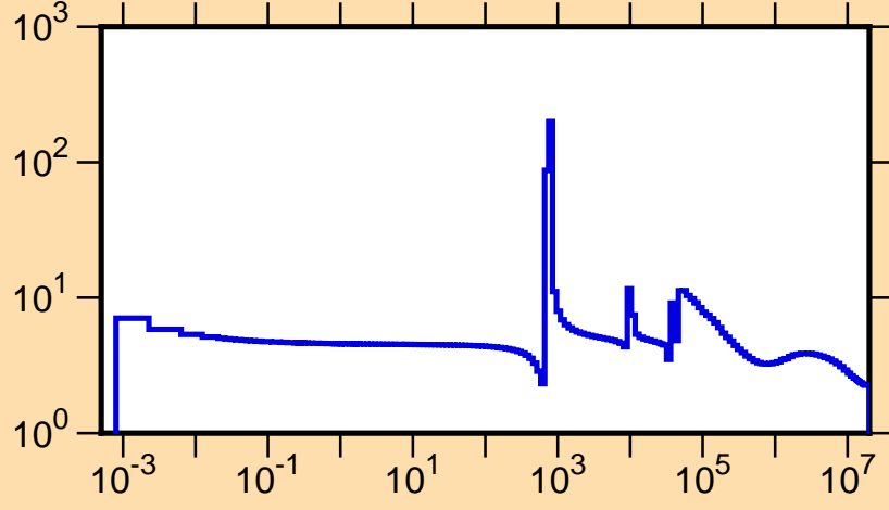
\sigma vs. E for ^{51}\text{Ti}(n,\text{tot.})
