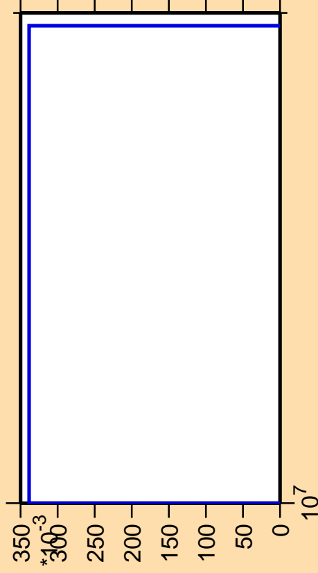
\Delta\sigma/\sigma vs. E for ^{51}\text{Ti}(n,2np)
