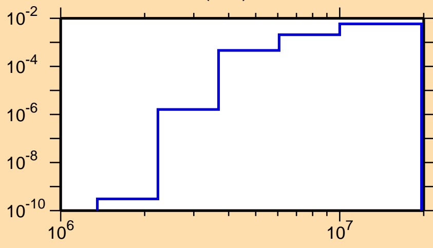
\sigma vs. E for ^{51}\text{Ti}(n,\alpha)
