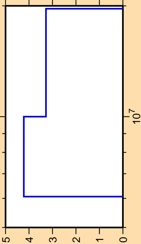
\Delta\sigma/\sigma vs. E for ^{51}\text{Ti}(n,2n)
