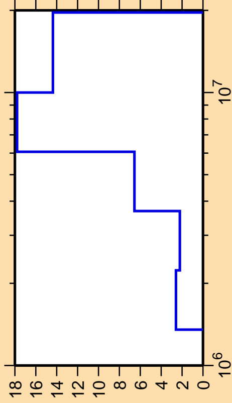
\Delta\sigma/\sigma vs. E for ^{51}\text{Ti}(n,n_4)
