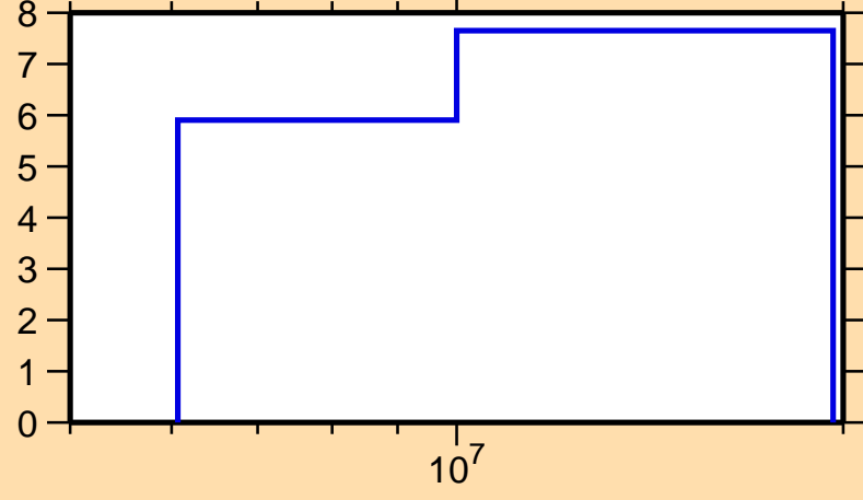
\Delta\sigma/\sigma vs. E for ^{51}\text{Ti}(n,\text{inel.})
