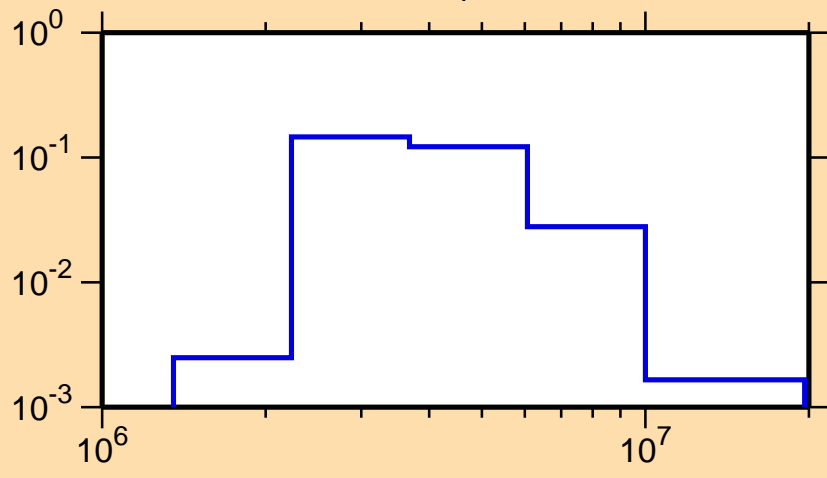
\sigma vs. E for ^{51}\text{Ti}(n,n_4)
